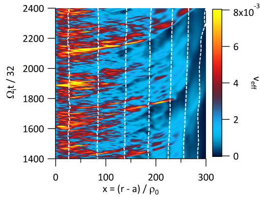
Figure 12. Effective ballistic transport velocity, the dashed white lines localise the zero contour of the zonal flow pattern, in the vicinity of the maximum shear.
