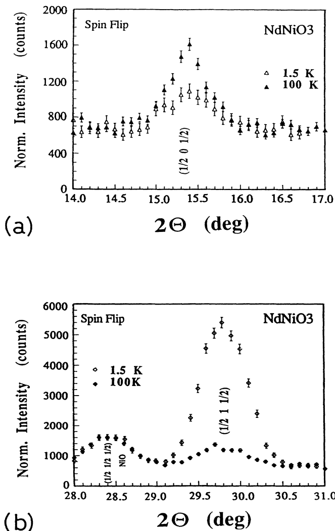
FIG. 4. Comparison of the 1.5 and 100 K spin-flip signals in NdNiO 3 for (a) the (\frac{1}{2}, 0, \frac{1}{2}) and (b) (\frac{1}{2}, 1, \frac{1}{2}) magnetic reflections (see explanation in the text).
