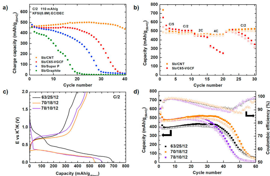
Fig. 2. a) Reversible capacity as a function of cycle number for the four Sb/C electrodes, b) Rate capability of Sb/DWCNT and Sb/C65/VGCF electrodes from C/5 to 4C rate, c) 1st cycle of Sb/DWCNT electrode with different weight ratios d) the corresponding capacity retention with CE.
