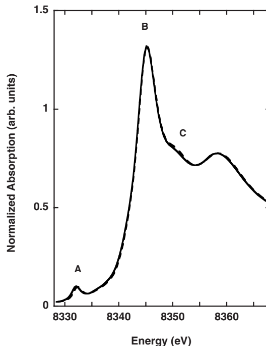
FIG. 2. Ni K -edge XANES simulation using the average crystallographic structure reported by neutron diffraction in the insulator (solid line) and metallic (dashed line) phases.
