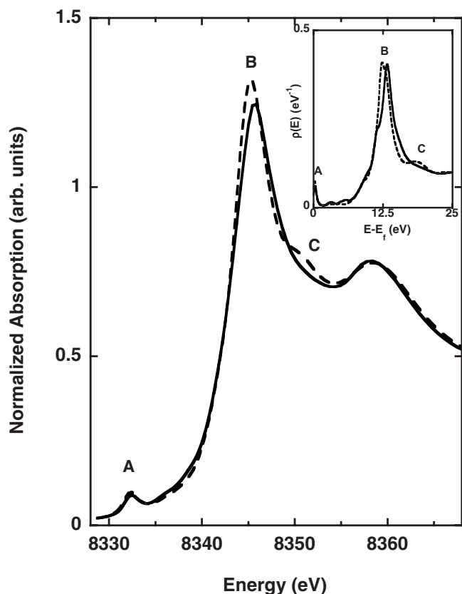
FIG. 3. Ni K -edge XANES simulation in the metallic (dashed line) and insulating (solid line) phases using orthorhombic symmetry and monoclinic symmetry groups respectively (dashed line). Inset: Ni p density of states as a function of energy, measured from the calculated Fermi level, for the orthorhombic structure (dashed line) and monoclinic structure (solid line).
