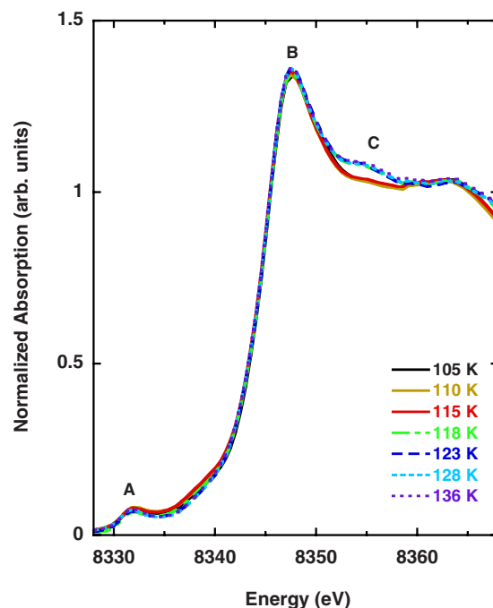
FIG. 1. (Color online) Normalized Ni K -edge XANES experimental data at different temperatures above (dashed lines) and below (solid lines) of metal-insulator transition. Quoted temperatures refer to nominal temperatures as explained in the text.
