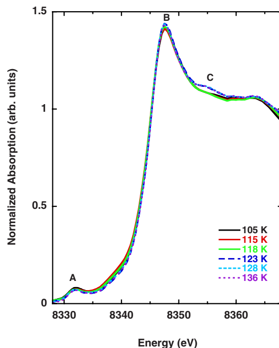
FIG. 4. (Color online) Ni K -edge XANES for ^{18}\text{O} \text{PrNiO}_3 at different temperatures above (dashed lines) and below (solid lines) of the metal-insulator transition. Quoted temperatures refer to nominal temperatures as explained in the text.
