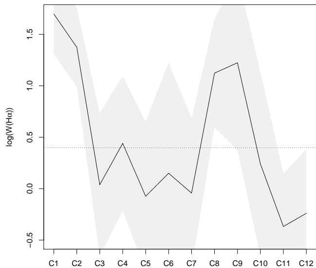
Fig. 13. Evolution of the median of W(H\alpha) for the cluster sample. Shaded regions show 1\sigma dispersion around median. The horizontal dotted line is for W(H\alpha)=2.5 (see text and Figs. 10, 11, 12).
