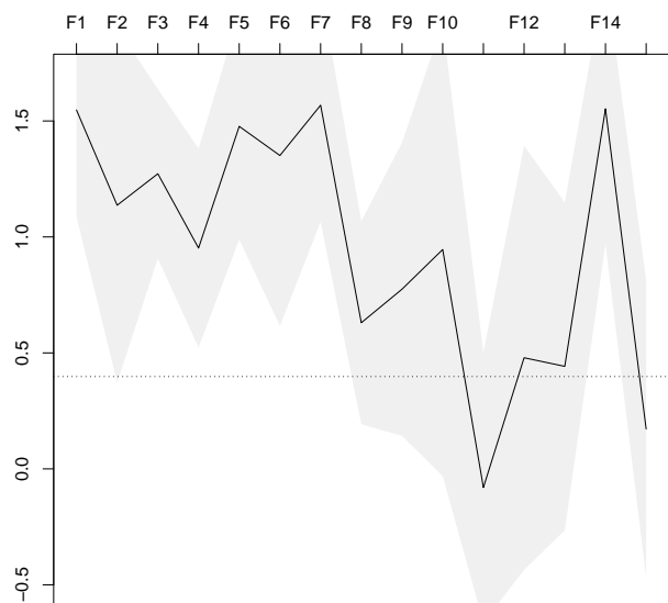
Fig. 13. Evolution of the median of W(H\alpha) for the cluster sample. Shaded regions show 1\sigma dispersion around median. The horizontal dotted line is for W(H\alpha)=2.5 (see text and Figs. 10, 11, 12).
