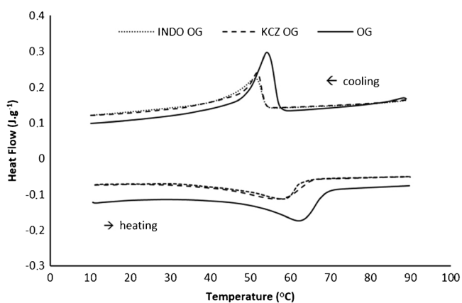
Fig. 3. DSC thermograms examples of unloaded and drug loaded (3% w/w) HSA (15% w/w) organogels
