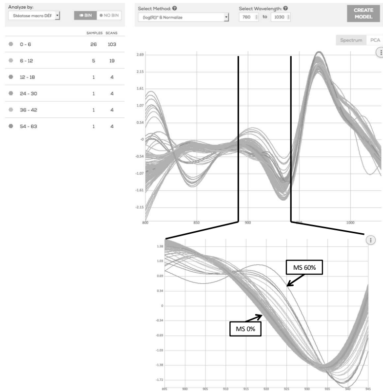
Spectra from the 35 selected livers during stage 1
