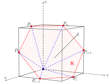
Figure 4: Interface polygon and intersection points in the context of VOFTOOLS.
