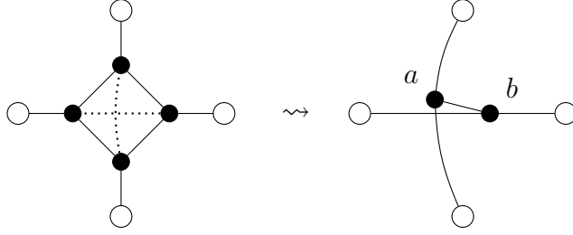
Figure 2: An example of the reduction from G to G' for (B).
