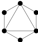
Figure 1: A negative answer to Question 1.2 for k = 1 .
