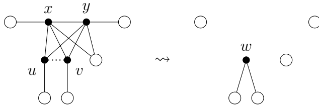
Figure 3: An example of the reduction from G to G_{uv} for (C).
