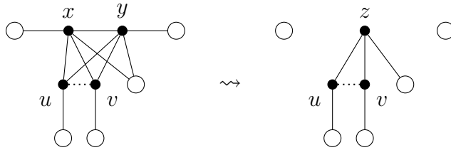
Figure 4: An example of the reduction from G to G' for (C).
