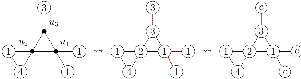
Figure 5: An example of the colouring extension when \omega(G) \geq 3 .
