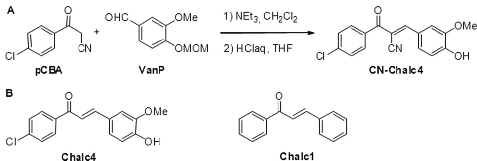
SCHEME 1. A, synthesis of CN-chalcone 4 (CN-Chalc4) following a Knoevenagel condensation of pCBA with 3-methoxy-4-(methoxymethoxy)benzaldehyde (VanP). B, structure of reference compounds chalcone 4 (Chalc 4) and unsubstituted chalcone (Chalc 1).
