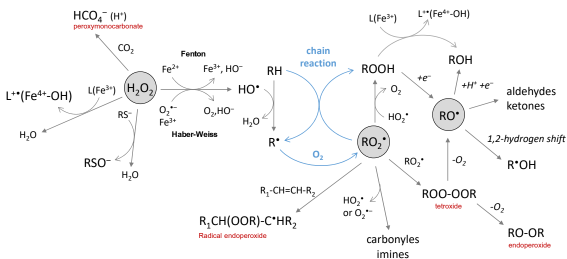
Figure 4. The chemical reactions of hydrogen peroxide, peroxy and alkoxyl radicals.
