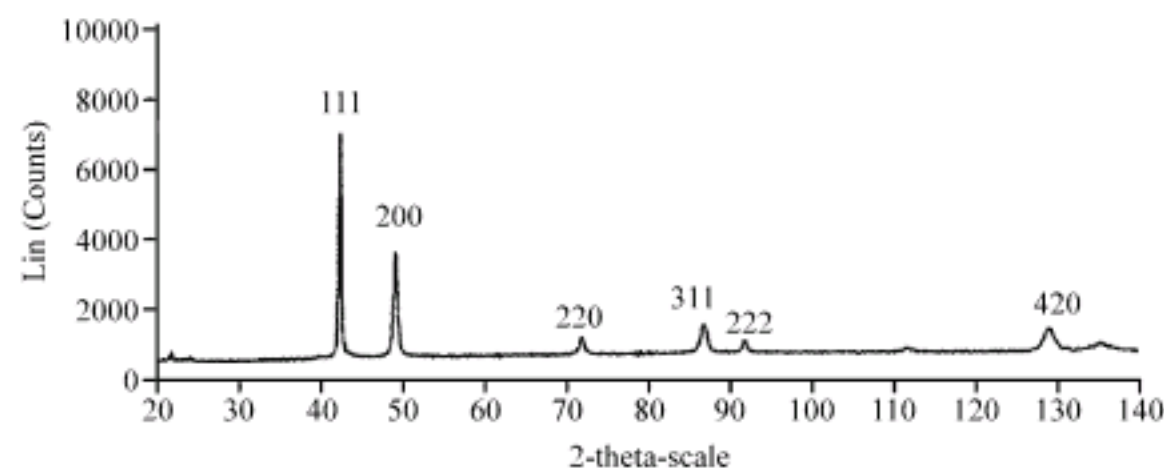
Fig. 5: The X-ray diffraction analyse of infiltrant Cu-Mn
