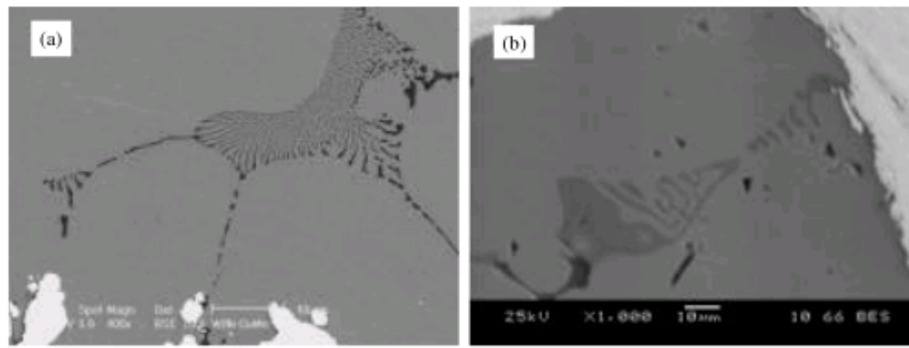
Fig. 9: BSE micrographies of intermetallic phase: (a) Mn_3P_2 in M1 grade, (b) Mn_2P in M2 grade
