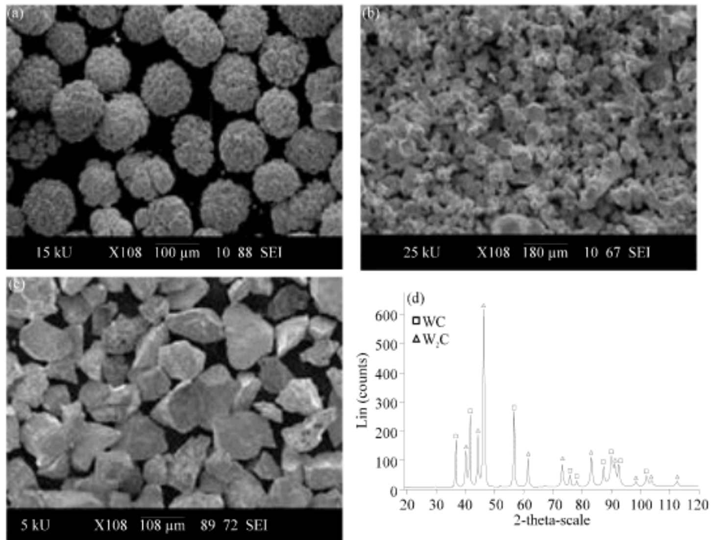
Fig. 2: SEM image of Ni powder (a), W powder (b), WC powder (c) and (d) X-ray diffraction analyse of WC powder
