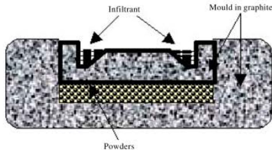
Fig. 1: Schematic representation of the infiltration process
