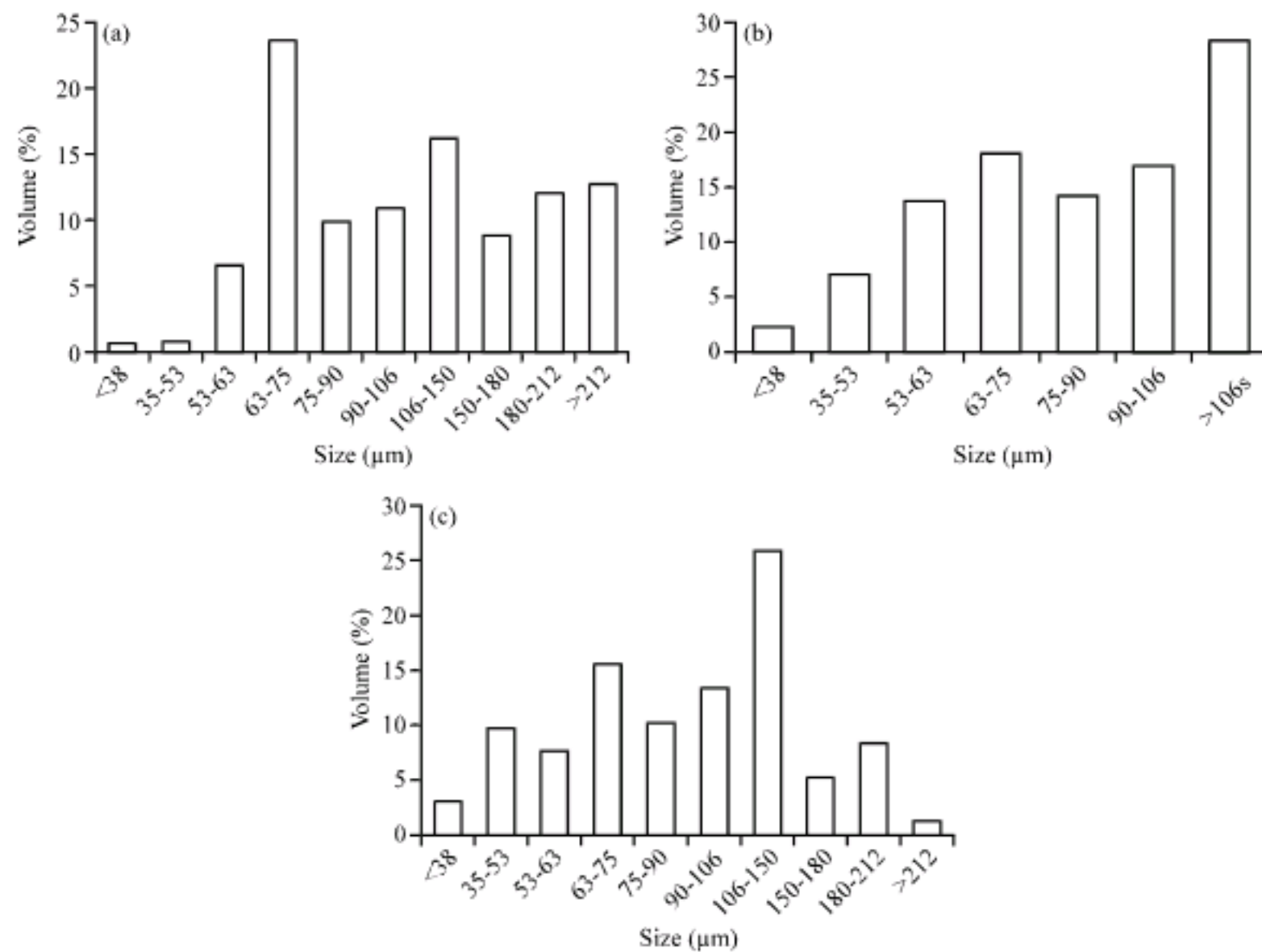
Fig. 3: Granulometric histogram of distribution for powders (a) WC, (b) W and (c) Ni according to the average size
