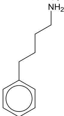
Scheme 1. Phenylbutylamine (PBA).
