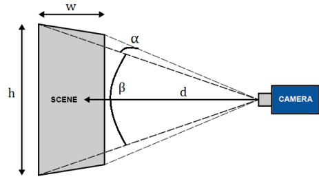
Fig. 3: Field of view of a camera
