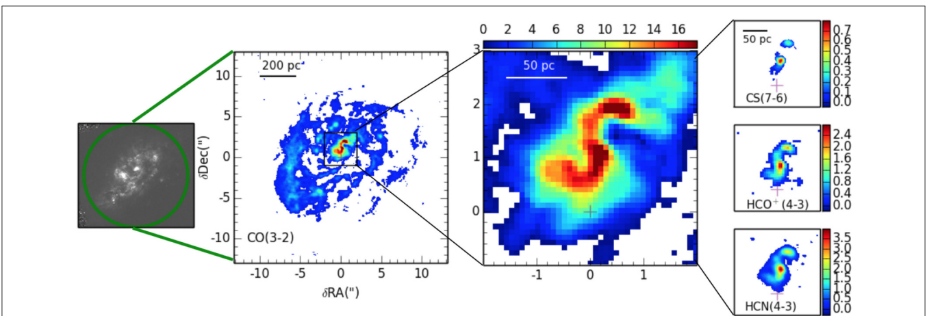
FIGURE 3 | From the left to the right panels: a WFC/F658N HST image followed by the 26'' diameter imaged area of CO(3-2) observations with ALMA. The next panels shows a zoom of the spiral trailing structure observed, and the subsequent plots show the same detection as seen in CS(7-6), HCO + (4-3), and HCN(4-3). All the intensity maps were clipped at >5\sigma .
