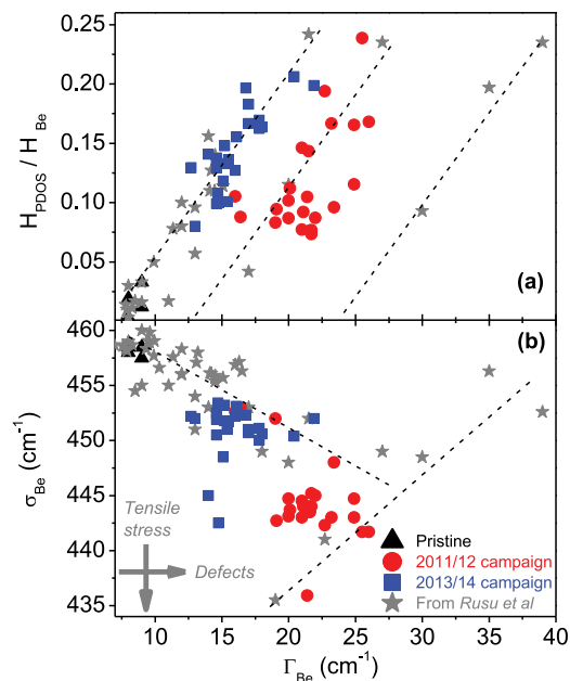
Fig. 4. Raman parameter plots characterizing the Be phase. (a) H_{\text{PDOS}}/H_{\text{Be}} as a function of \Gamma_{\text{Be}} . (b) \sigma_{\text{Be}} as a function of \Gamma_{\text{Be}} . Data in grey and black from [18] have been added for comparison. Lines are guides for the eyes. (For interpretation of the references to colour in this figure legend, the reader is referred to the web version of this article.)
