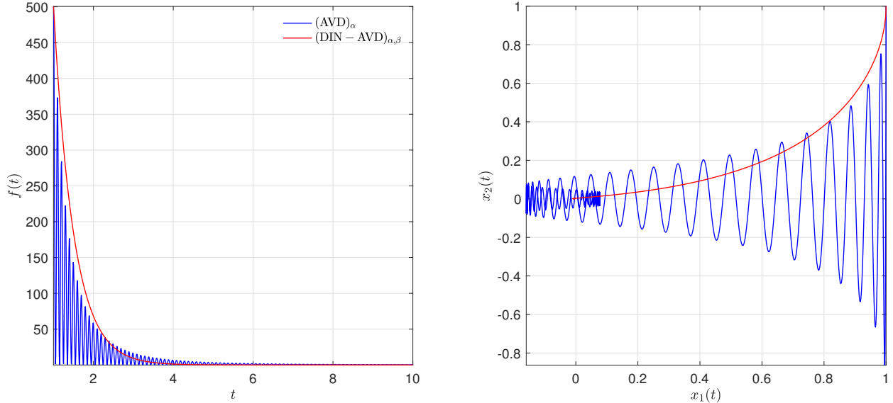
FIGURE 1. Evolution of the objective (left) and trajectories (right) for (\text{AVD})_\alpha ( \alpha = 3.1 ) and (\text{DIN-AVD})_{\alpha,\beta} ( \alpha = 3.1, \beta = 1 ) on an ill-conditioned quadratic problem in \mathbb{R}^2 .
