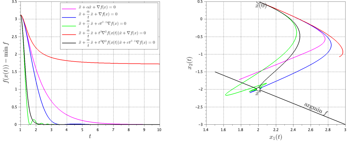
FIGURE 2. Convergence of the objective values and trajectories associated with the system (\text{DIN-AVD})_{\alpha,\beta,b} for different choices of \beta(t) and b(t) .
