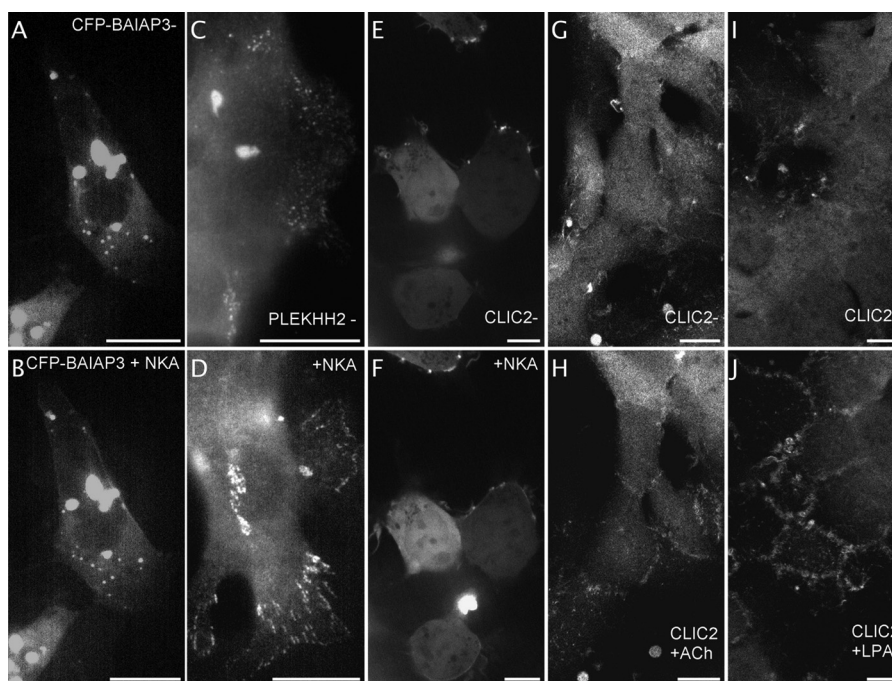
FIG. 7. Identification of fluorescent proteins of unknown function that respond to NK2 receptor activation by a change in localization. Images extracted from videos of CFP-BAIAP3 expressing NK2R-HEK cells before (A) and within seconds after NKA activation (B, from video 1 out of 5). Representative epifluorescence images acquired close to the slide of fixed PLEKHH2-YFP expressing NK2R-HEK cells before (C) and after 3 h NKA activation (D), n = 3 independent experiments. Images extracted from videos of CLIC2-YFP expressing NK2R-HEK cells before (E) and 2 min after NKA activation (F, from video 2 out of 7 videos, 4 cells displayed out of 8). Images extracted from video1 of HEK293 cells stably expressing CLIC2-mYFP before (G) and 20 min after activation of endogenous Gq-coupled muscarinic M3 receptors with 10 \mu\text{M} ACh (H) n = 3 independent experiments. Images extracted from video1 of HEK293 cells stably expressing CLIC2-mYFP before (I) and 25 min after activation of endogenous G12-coupled lysophosphatidic acid receptors with 1 \mu\text{M} LPA (J). n = 2 independent experiments. Scale bar 5 \mu\text{m} .
