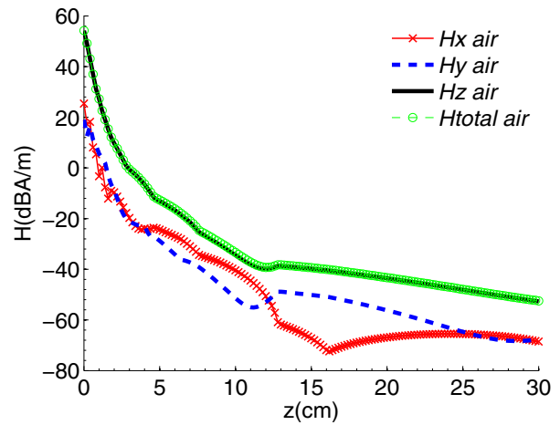
Figure 13. Magnetic field components and total magnetic field of the loop antenna versus the z distance in the air
