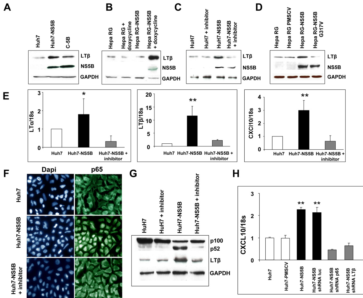
Figure 7. NS5B enzymatic activity is required for activation of lymphotoxin expression and signaling. (A) Expression of LTβ protein in exponentially growing Huh7 cells, Huh7 stably expressing NS5B (Huh7-NS5B) and Nneo/C-5B replicon (C-5B) (B) Expression of LTβ protein in HepaRG and HepaRG-NS5B doxycycline-inducible cells (HepaRG-iNS5B). (C) Expression of LTβ protein in exponentially growing Huh7 cells and in Huh7 stably expressing NS5B, treated with the NS5B polymerase inhibitor 2'-C-Methylcytidine, as indicated. (D) Expression of LTβ protein in HepaRG, HepaRG-PMSCV, HepaRG-NS5B and HepaRG-NS5B G317V. (E) RT-qPCR analysis of LTα, LTβ, LTβR and CXCL10 mRNA expression in Huh7 and Huh7-NS5B treated or not by 2'-C-Methylcytidine. 18S rRNA served as normalization standard. (F) Immunofluorescence analysis of p65 nuclear translocation in Huh7 cells and Huh7-NS5B treated or not with 2'-C-Methylcytidine. (G) Expression of p100, p52 and LTβ proteins in Huh7 cells and Huh7 stably expressing NS5B treated or not with 2'-C-Methylcytidine. (H) RT-qPCR analysis of CXCL10 mRNA expression. Parental and NS5B-expressing Huh7 cells were transduced with retroviral vectors encoding shRNA directed against p65, LTβ or Firefly luciferase as control. Where appropriate, results are presented as mean±SEM of three separate experiments (student test, *p<0.01, **p<0.001). doi:10.1371/journal.ppat.1003234.g007
