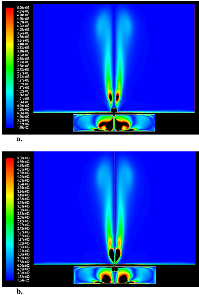
Figure 9. Iso-contours of vorticity – k-ε model. a) t/T = 0.25 , b) t/T = 0.75
