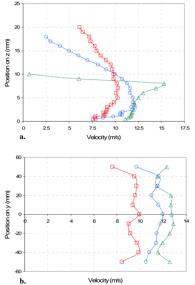
Figure 10. Wall jet velocity profiles for 3 sections a) z profile, b) y profile \Delta : 3mm, \circ : 60 mm, \square : 120mm
