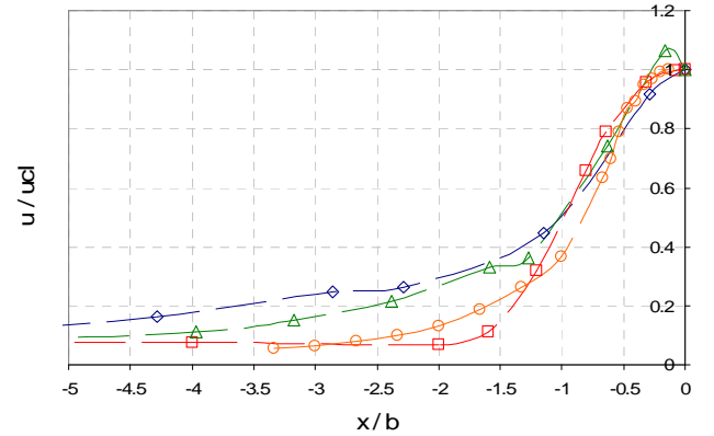
Figure 8. Distribution of time-averaged velocity at z/h = 10 with f = 1100 Hz, h = 500 \mu m, pressure amplitude : 2 \times 10^3 Pa \diamond : Laminar, \square : k-\epsilon , \triangle : k-\omega , \circ : Experimental
