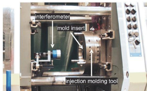
Fig. 12. An on-machine Twyman-Green interferometer with a fast Fourier transform (FFT) algorithm for an injection molding machine [201].
