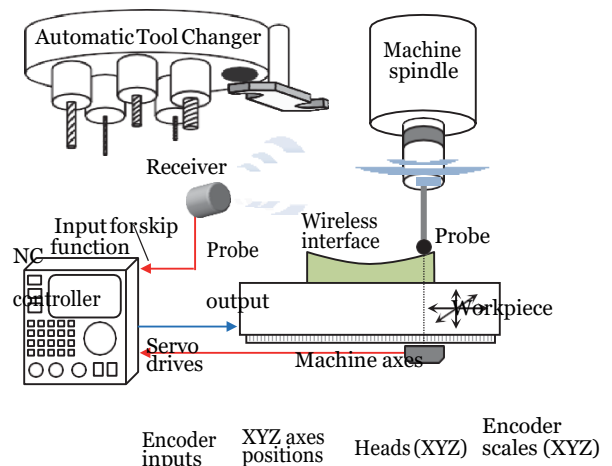
Fig. 33. Interfaces in an NC controller integrated probe-scan system.
