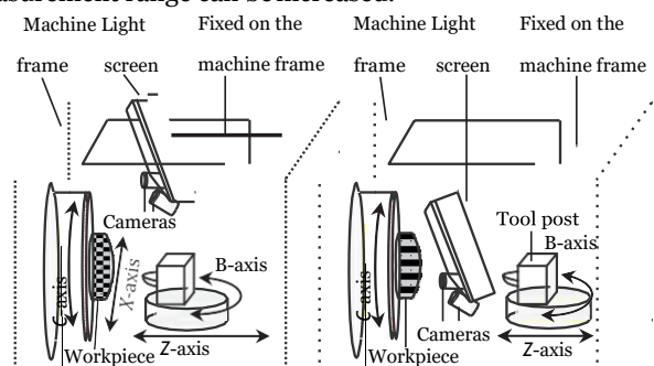
Fig. 16. Fully machine integrated setup of a PMD in stand-by position (left) and in measurement position (right) (modified from [48]).
