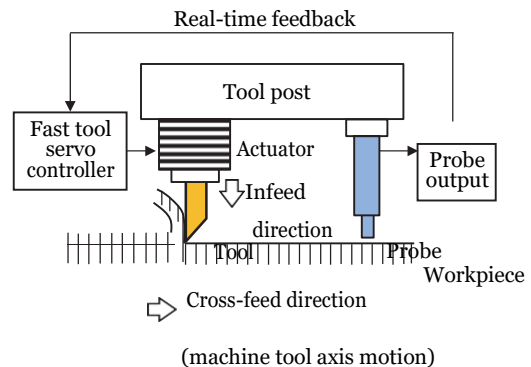
Fig. 38. Real-time feedback to compensation machining (modified from [229]).
