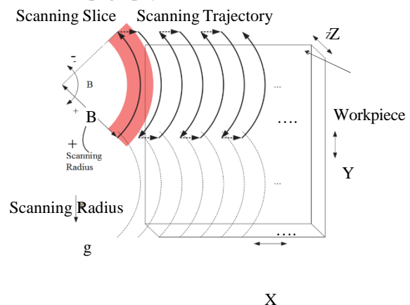
Fig. 32. Scanning strategy of the on-machine metrology [151].
