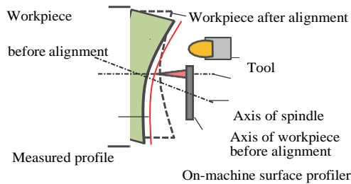
Fig. 6. On-machine surface metrology for initial alignment of workpiece.
