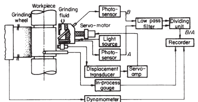
Fig. 30. In-process surface metrology as proposed by Inasaki [97].
