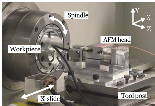
Fig. 23. An on-machine AFM head with a linear encoder [60].
