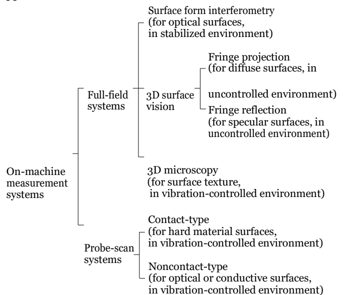
Fig. 8 Measurement systems for on-machine surface metrology.
