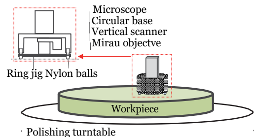
Fig. 18. A point source microscope located on the workpiece surface for passive anti-vibration (modified from [182]).
