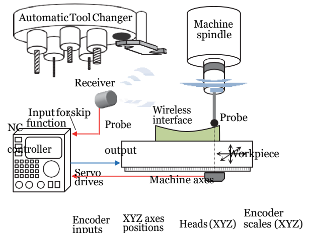
Fig. 33. Interfaces in an NC controller integrated probe-scan system.
