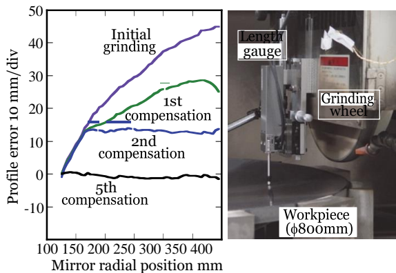
Fig. 39. On-machine measurement and compensation grinding of a SiC aspheric mirror workpiece through feedback to machine NC [208].
