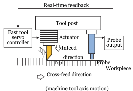
Fig. 38. Real-time feedback to compensation machining (modified from [229]).
