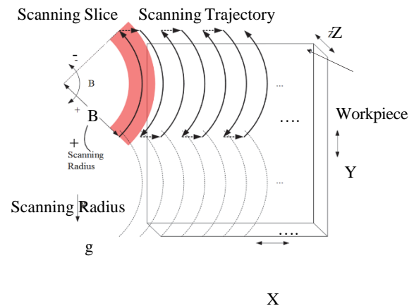
Fig. 32. Scanning strategy of the on-machine metrology [151].
