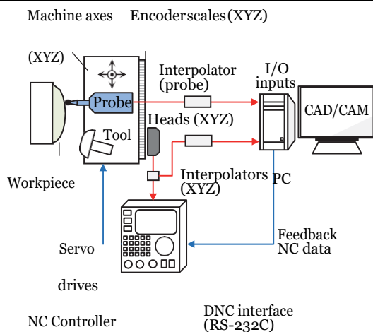
Fig. 34. Interfaces in a PC-based on-machine surface metrology system (modified from [174]).
