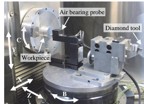
Fig. 21. An on-machine air bearing probe [259].
