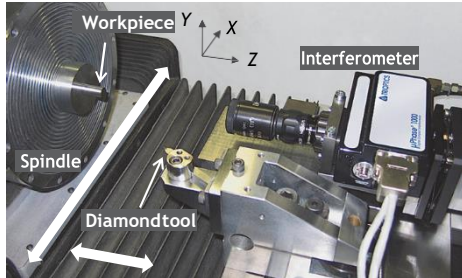
Fig. 10. An on-machine Twyman-Green dynamic interferometer [228].
