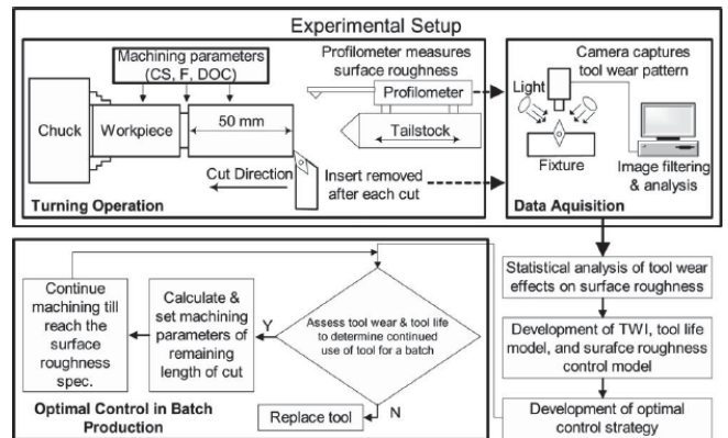
Fig. 29. On-machine surface metrology for roughness measurements as proposed by Kwon [130].
