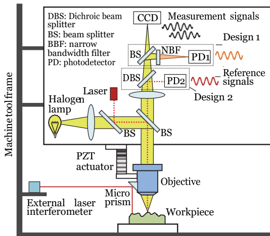
Fig. 19. External and internal reference displacement interferometers in 3D microscopy for active anti-vibration (modified from [200][22]).
