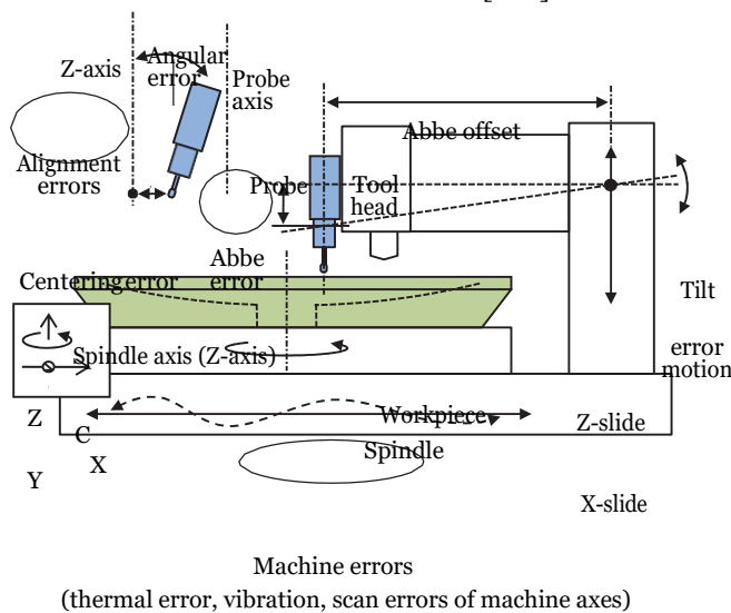
Fig. 25 Error sources in integration of probe into machine tool.
