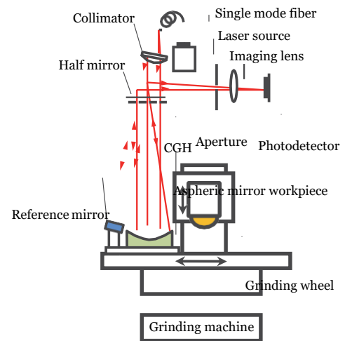
Fig. 11. An on-machine common-path interferometry system for a horizontal surface grinding machine [120].
