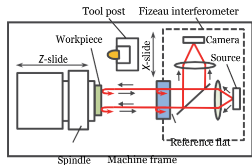
Fig. 9. Schematic of a Fizeau interferometer on a diamond turning machine (modified from [181]).
