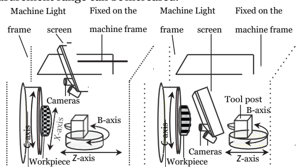
Fig. 16. Fully machine integrated setup of a PMD in stand-by position (left) and in measurement position (right) (modified from [48]).
