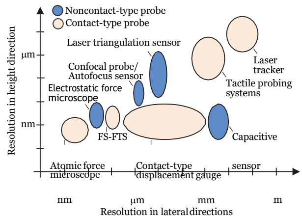
Fig. 20. Probes for on-machine surface metrology.
