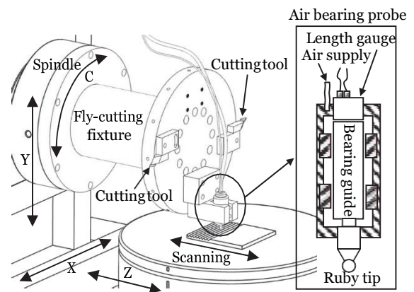
Fig. 40. On-machine measurement and compensation cutting of vee-grooves through feedback to adjustment of tool position and orientation [257].
