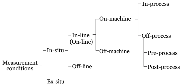
Fig. 1. Conditions of surface metrology for precision manufacturing.
