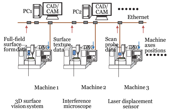
Fig. 35. Ethernet interfaces for next generation on-machine surface metrology network.
