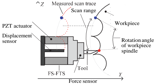
Fig. 22. FS-FTS used for on-machine measurement of micro-structured surface (modified from [62]).
