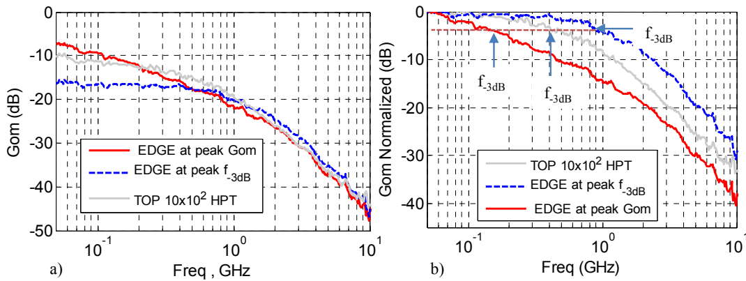
Figure 13: a) The opto-microwave responsivity versus frequency of edge and top ( 10 \times 10 \mu\text{m}^2 ) illuminated HPT. b) The normalized opto-microwave responsivity versus frequency for edge illuminated HPT at x=-4 \mu\text{m} and z=0 \mu\text{m} and x=y=0 \mu\text{m} , and top illuminated HPTs at its peak detection.
