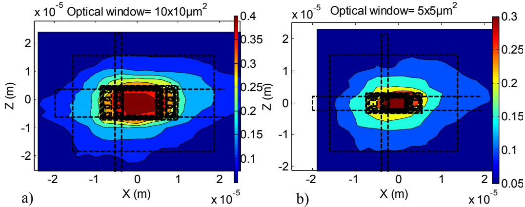
Figure 8: -3dB cutoff frequency (in GHz) topological maps at V_{ce}=3V and V_{be}=0.857V a) 10 \times 10 \mu m^2 optical window HPT, b) 5 \times 5 \mu m^2 optical window HPT.
