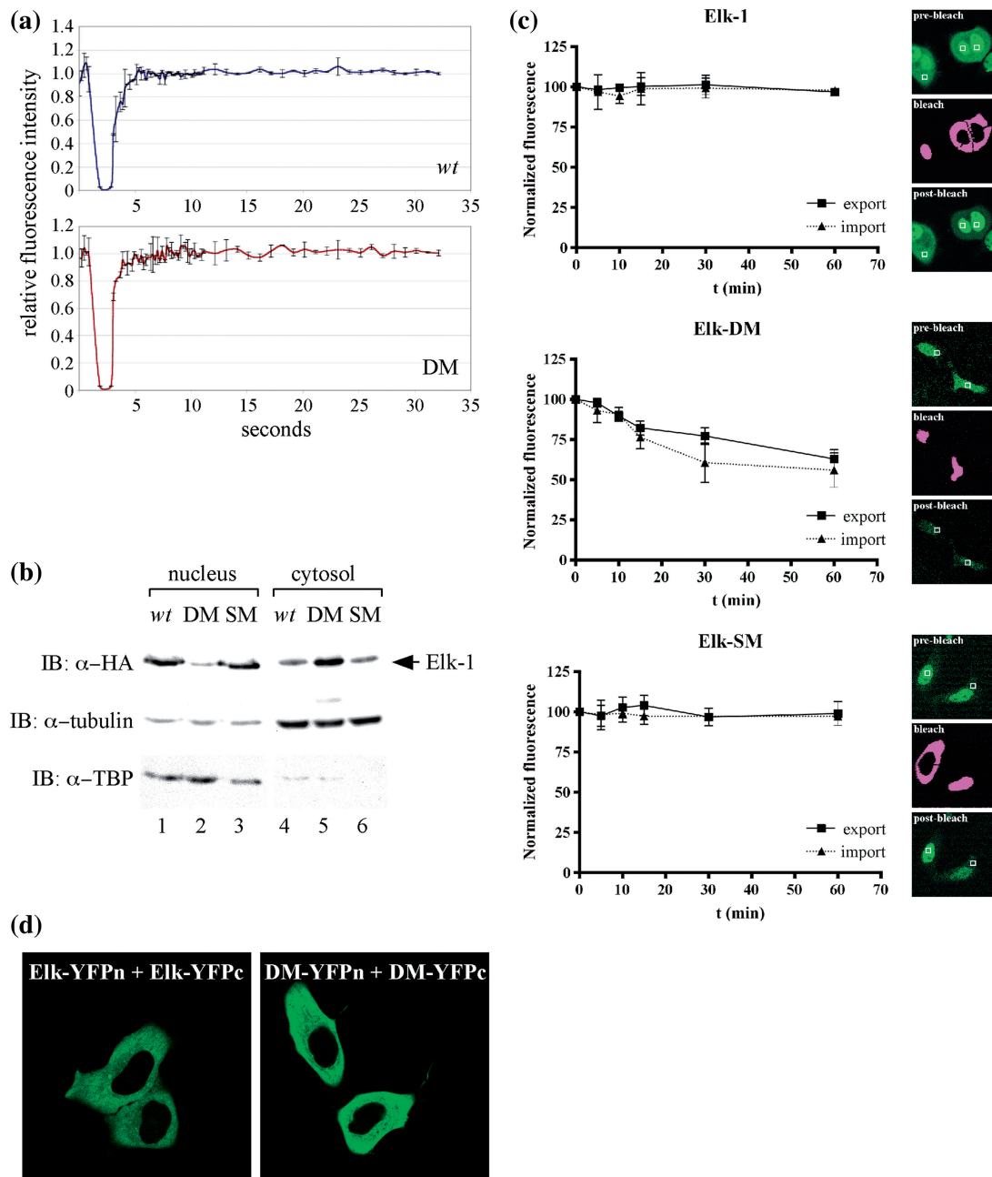
Figure 7. Mobility and accumulation of Elk-1 in HeLa nuclei. (a) HeLa cells cultured in glass-bottomed petri dishes were transfected with vectors for Elk-GFP or Elk-DM-GFP and after recovery for 24 h in full medium, mobility of Elk-1 was determined by FRAP. Data presented are average values ( \pm SE) for recovery measured on 10 individual cells from one representative experiment. (b) Nuclear and cytosolic fractions were prepared from HEK293 cells transfected with expression vectors for Elk-1 (lanes 1 and 4) Elk-DM (lanes 2 and 5) and Elk-SM (lanes 3 and 6) were separated by SDS-PAGE and analysed by immunoblotting with the antibodies indicated. (c) HeLa cells cultured in glass-bottomed petri dishes were transfected with vectors for Elk-GFP, Elk-DM-GFP or Elk-SM-GFP and after recovery for 24 h in full medium, mobility of Elk-1 was followed by FLIP over 60 min. Data are compiled from measurements on five individual cells for each time course (error bars show SEM). Panels show examples of cells prior to bleach (upper), immediately after bleach (middle) and 60 min post bleach (lower). (d) Fluorescence images of live HeLa cells 16 h post-transfection with expression vectors for Elk-YFPn and Elk-YFPc (left panel) or Elk-DM-YFPn and Elk-DM-YFPc (right).
