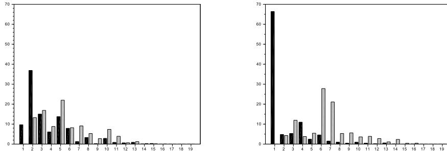
Figure 1: The incidence of diagonal perturbations on the terms of the bound (5)
