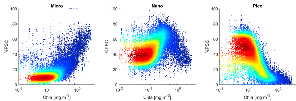
Figure 12. Interpigment relationships represented as percentage of phytoplankton size classes (microphytoplankton, nanophytoplankton, and picophytoplankton) in function of Chla, calculated within the neurons of the SOM-pigments. ( \%Micro = 1.41(NFuco + Perid)/\Sigma DP , \%Nano = (Xn * 1.27Hex + 1.01Chlb + 0.35But + 0.6Allo)/\Sigma DP , \%Pico = 1 - (\text{micro} + \text{nano}) ; with \Sigma DP = 1.41Fuco + 1.41Perid + 1.27Hex + 1.01Chlb + 0.35But + 0.6Allo + 0.86Zea and Xn indicates a proportion of nanoplankton contribution in Hex (Hirata et al., 2011; Uitz et al., 2006).
