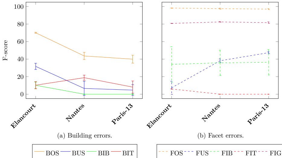
Figure 12. Mean F-score and standard deviation for the generalization study per test zone.
