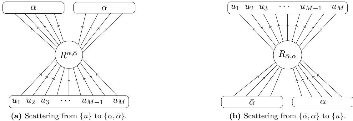
Figure 13. Multi-scattering R -matrices in (E.83) and (E.86).
