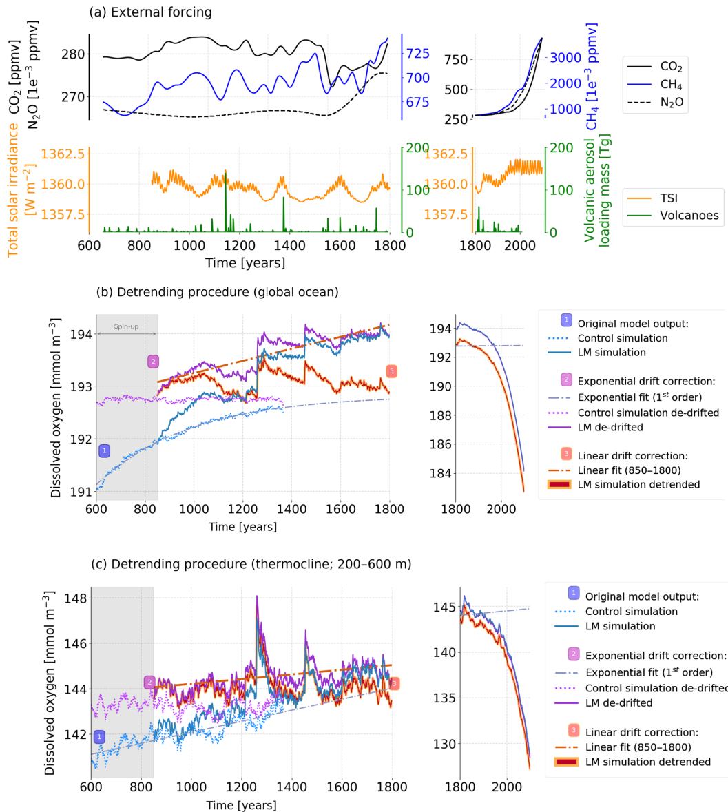
Figure A1. (a) Time series of the main external forcings applied to the forced simulation: total solar irradiance ( W m^{-2} ) at the top of the atmosphere in orange, stratospheric volcanic aerosol load (Tg) in green and the greenhouse gases CO 2 (solid black line), N 2 O (dashed black line) and CH 4 (solid blue line) (ppmv). Illustration of the two-step procedure to remove model drift and millennial-scale trends at each grid point shown in (b) the global mean ocean and (c) the thermocline (200–600 m). The original, annually averaged outputs from the control (CTRL) and the forced simulations are shown by dashed and solid blue lines, respectively (1). The results of the CTRL are fitted by an exponential function with one timescale and extrapolated towards equilibrium (dashed line). The exponential curve is subtracted from and the equilibrium value added to the original outputs to obtain the purple curves (2) (dotted: CTRL, solid: forced simulation). The remaining multi-millennial trend in the forced simulation is removed using a linear fit (850–1800 CE), leading to the red curve (3).
