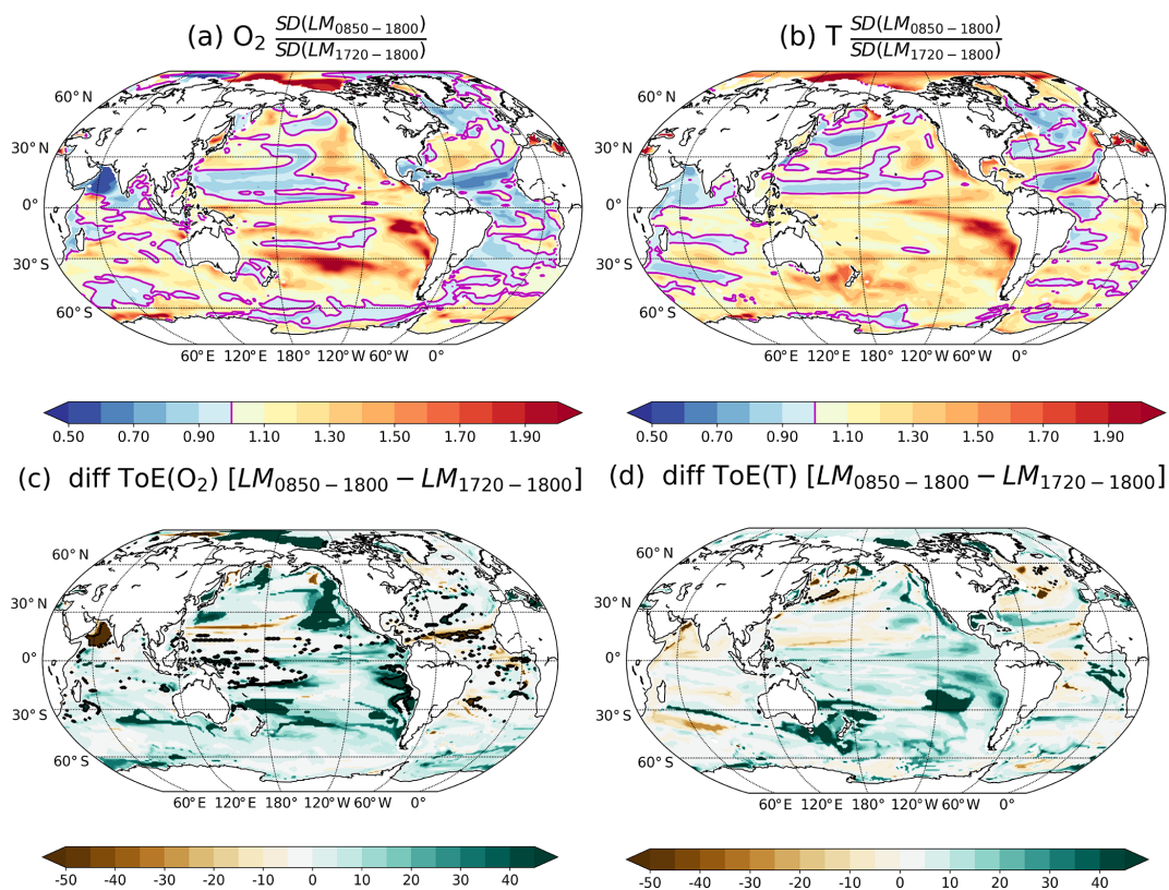
Figure A6. Ratio of the SDs of the forced simulation computed over the period 850–1800 CE and over the period 1720–1800 CE for (a) O 2 and (b) T. Difference of ToE using the SD of the forced simulation over the period 850–1800 CE minus the ToE using the SD of the same simulation but over the pre-industrial period (1720–1800 CE) for (c) O 2 and (d) T. The magenta contours highlight the ratio equal to 1, i.e. where SDs are equal. SDs are computed from annually and vertically averaged values between 200 and 600 m.
