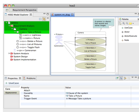
Figure 16: The Workbench
