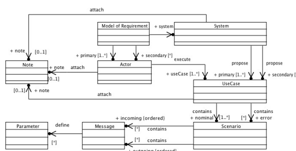
Figure 2: Requirement Metamodel
