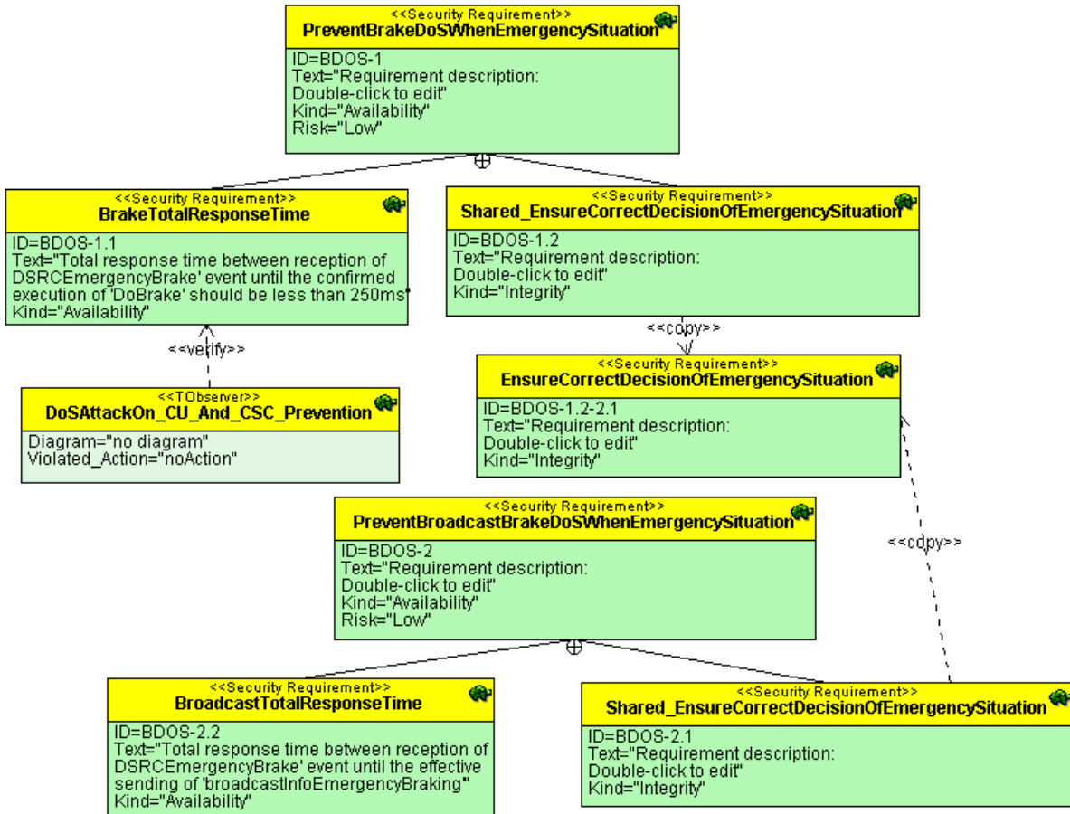
Fig. 2. Excerpt of the requirement diagram: Denial of Service related security requirements
