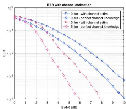
Fig. 6. BER over TV channels for block-based CPM
