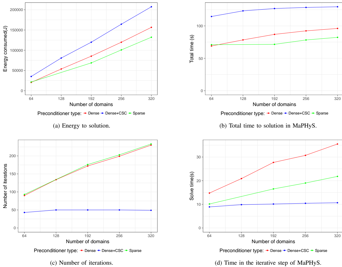
Fig. 4. Time and energy performance for MAPHYS .
