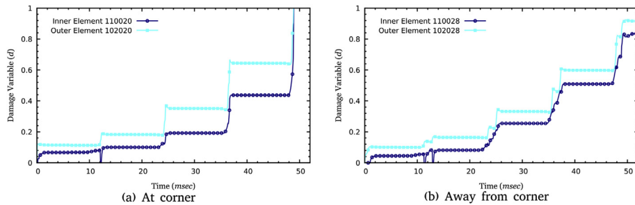
Fig. 10. Damage variable, d , as a function of time ( t_s = 1.5 mm).
