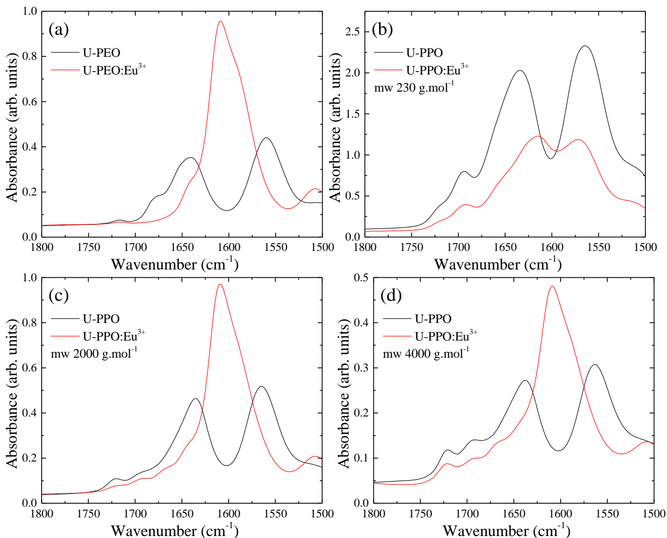
Figure 2: (2-column fitting image) Effect of \text{Eu}^{3+} doping on the amide I and II regions of the FTIR spectra of OIH films for (a) U-PEO (mw = 1900 \text{g}\cdot\text{mol}^{-1} ) and for U-PPO with mw of (b) 230, (c) 2000, and (d) 4000 \text{g}\cdot\text{mol}^{-1} .
