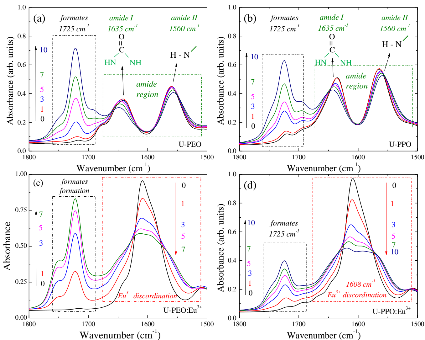
Figure 3: (2-column fitting image) Room temperature IR spectra from 1800 to 1500 \text{cm}^{-1} of the OIH films during photooxidation: (a) U-PEO, (b) U-PPO, (c) U-PEO: \text{Eu}^{3+} , and (d) U-PPO: \text{Eu}^{3+} .
