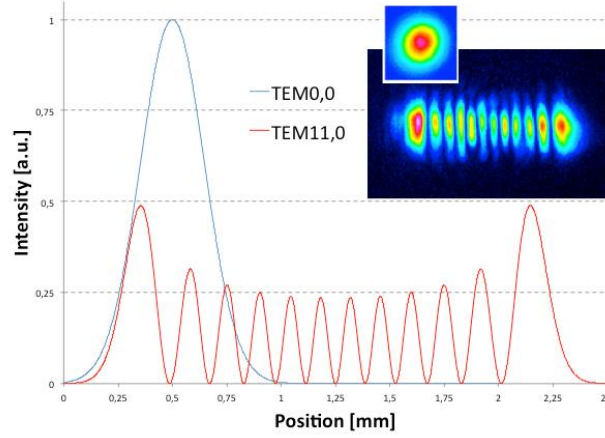
FIG. 7. High order mode Q-switched operation: enhancement of the beam size at normalized energy.
