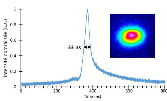
FIG. 9. Temporal and spatial profiles of the output laser, with an energy of 263 \mu\text{J} . Pump pulse duration of 250 \mu\text{s} with the 80% initial transmission saturable absorber and the 10% transmission output coupler, R = 500 mm. Cavity length = 80 mm.
