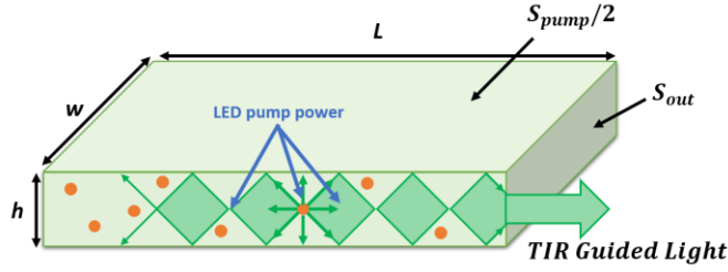
FIG.1. Schematic representation of a Ce:YAG Luminescent concentrator. 450 nm pump light is absorbed by \text{Ce}^{3+} ions, 550 nm reemitted light is guided by TIR toward the edge of the concentrator.
