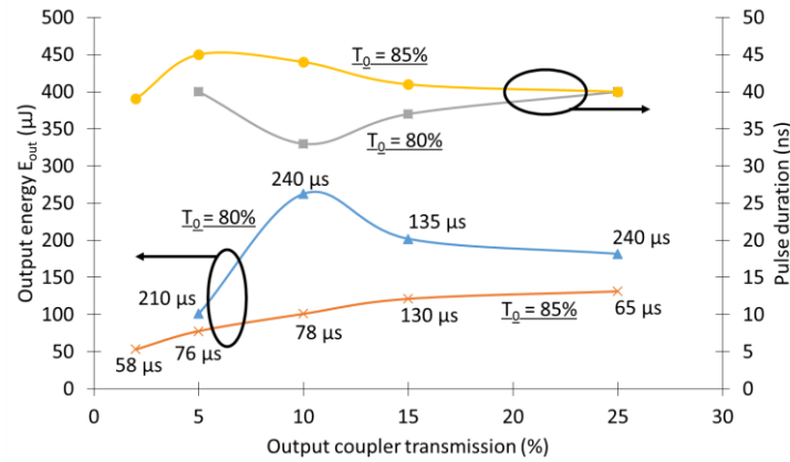
FIG. 8. Single-mode output energy and pulse duration in Q-switched operation as a function of the output coupler transmission, for each saturable absorber ( T_0=80\% and T_0=85\% ). Build-up time is indicated on the energy curves. The cavity length is 80 mm.
