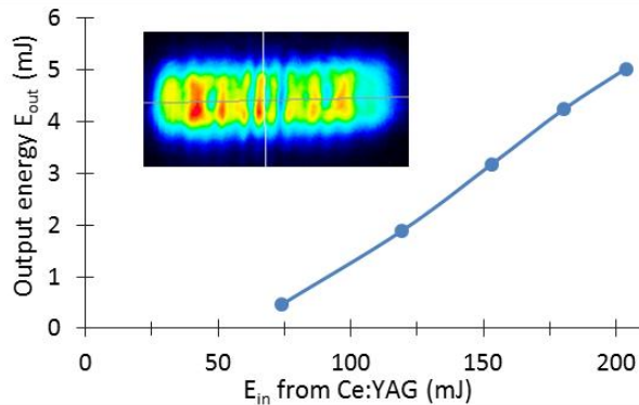
FIG. 5. Laser output energy in free running operation versus LC energy. LED are pulsed at 5 A during 250 \mu s at a frequency of 10 Hz. The cavity is 80 mm long with an output coupler having a radius of curvature of 500 mm and a transmission of 25%. Inset: Spatial profile at 5 A. The mode size is 2 mm by 0.75 mm, laser crystal facet being 2.5 mm by 1 mm.
