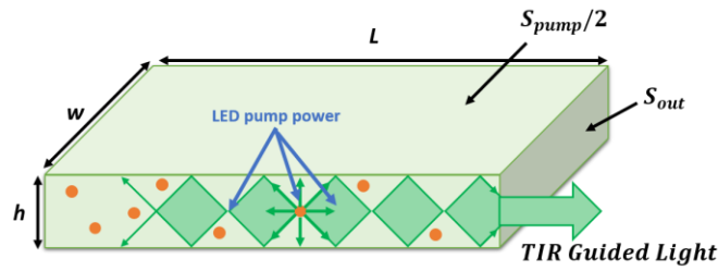
FIG.1. Schematic representation of a Ce:YAG Luminescent concentrator. 450 nm pump light is absorbed by Ce^{3+} ions, 550 nm reemitted light is guided by TIR toward the edge of the concentrator.
