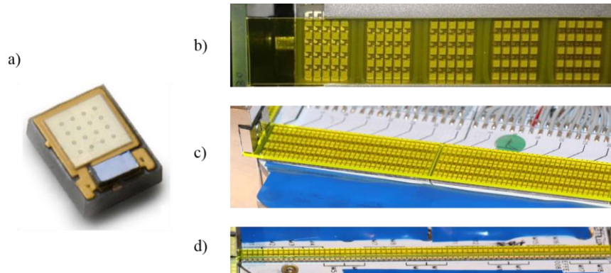
FIG.2. a) Picture of CSP LED, b) previous concentrator [9] and new ones : c) width of 14 mm and d) with of 2.5 mm.
