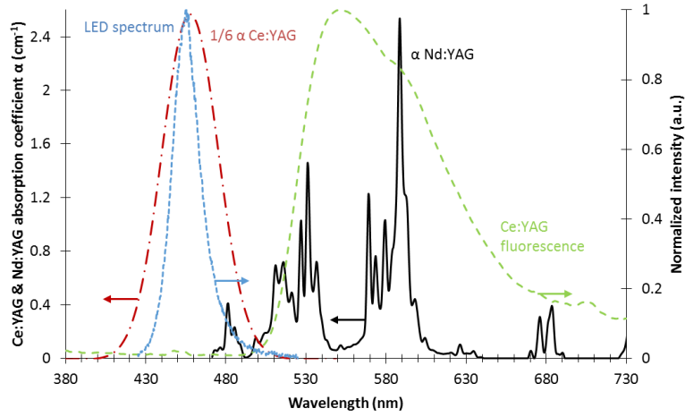
FIG. 3. Ce:YAG (red), Nd:YAG (black) absorption coefficient, emission spectra of Ce:YAG (green) and LED (blue) in the pulsed regime (250 \mu s, 5 A, 10 Hz, room temperature).
