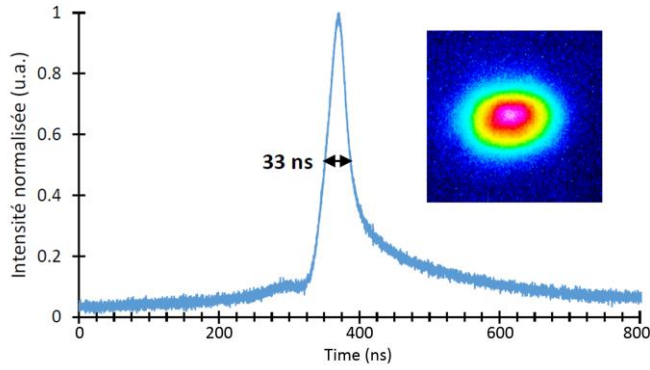
FIG. 9. Temporal and spatial profiles of the output laser, with an energy of 263 \mu\text{J} . Pump pulse duration of 250 \mu\text{s} with the 80% initial transmission saturable absorber and the 10% transmission output coupler, R = 500 mm. Cavity length = 80 mm.
