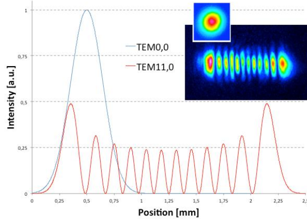
FIG. 7. High order mode Q-switched operation: enhancement of the beam size at normalized energy.
