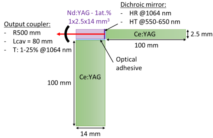
FIG. 4. Setup of the experiment. LEDs are placed above and underneath the Ce:YAG concentrators.
