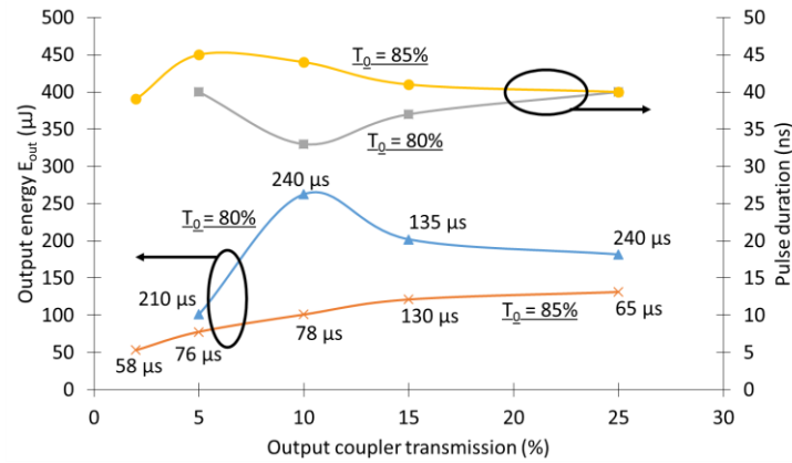
FIG. 8. Single-mode output energy and pulse duration in Q-switched operation as a function of the output coupler transmission, for each saturable absorber (T 0 =80% and T 0 =85%). Build-up time is indicated on the energy curves. The cavity length is 80 mm.
