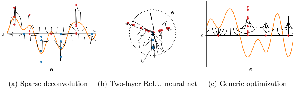
Figure 1: Three examples of conic particle gradient descents (Algorithm 1). Trajectories of particles in \Omega in black and their limits in red (positive mass) or blue (negative mass).
