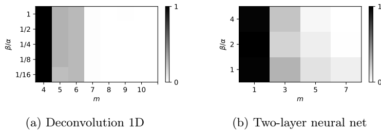
Figure 4: Effect of m and \beta/\alpha on the excess loss after a fixed large number of iterations ( \lambda fixed). The shades go from white (lowest objective achieved) to black (highest).
