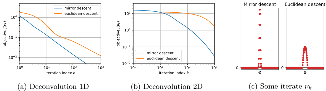
Figure 5: Comparison of mirror ( h(r) = r^2 ) and euclidean ( h(r) = r ) dynamics when \beta = 0 .
