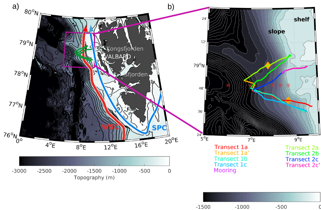
Figure 1. (a) Bathymetry from International Bathymetric Chart of the Arctic Ocean ( https://www.ngdc.noaa.gov/mgg/bathymetry/arctic/arctic.html ) along the west continental slope of Svalbard. Green lines are the SeaExplorer glider trajectory in July 2017. Black lines are bathymetry. (b) Zoom on the glider trajectory (purple box). Each color corresponds to a transect. Moorings at 78.5°N from the Alfred Wegener Institute (AWI) (Beszczynska-Möller et al., 2015) are located with orange stars (F1 to F5). The yellow diamonds indicate the lens locations. SPC = Spitsbergen Polar Current; WSC = West Spitsbergen Current.
