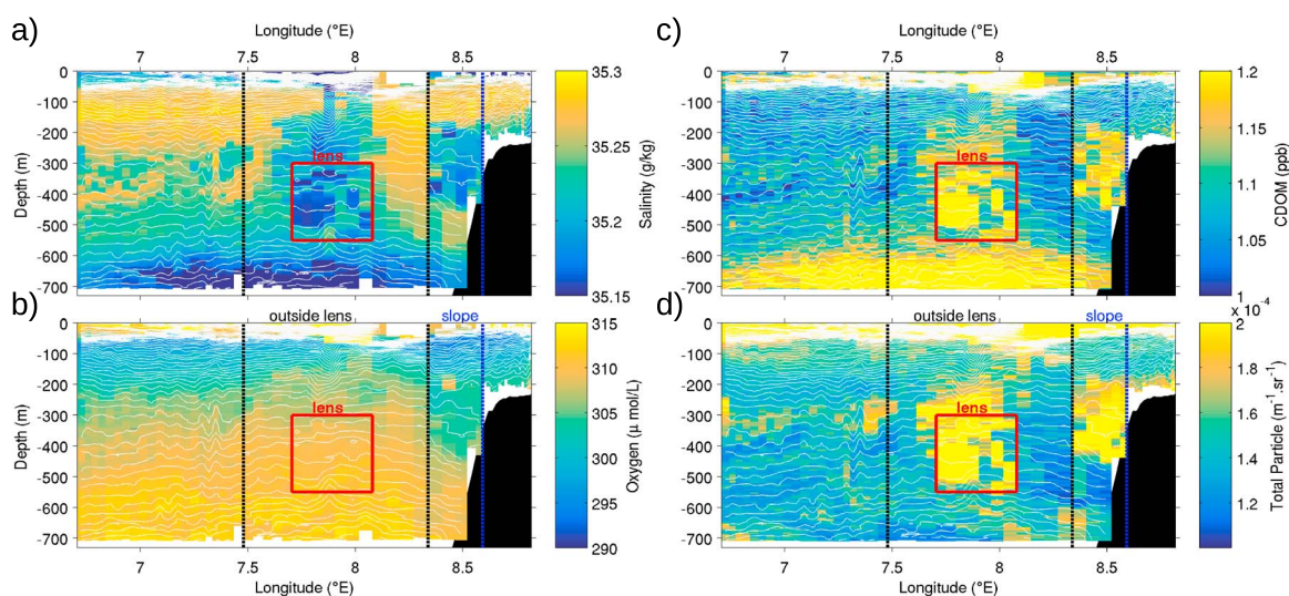
Figure 7. Same as Figure 4 but for transect 2a. CDOM = colored dissolved organic matter; ppb = parts per billion.
