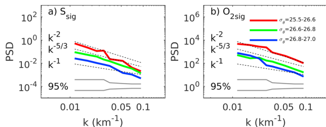
Figure 9. Density power spectra of isopycnal salinity (a) and dissolved oxygen (b) between 18^\circ W and 23^\circ W (C1, C2, D1 sections) within the \sigma_\theta = 25.5 – 26.6 (red), 26.6 – 26.8 (green), and 26.8 – 27 (blue) \text{kg/m}^3 isopycnal layers. The k^{-1} , k^{-5/3} , and k^{-2} slopes are superimposed (dashed lines). The 95% confidence interval is indicated by grey solid lines.
