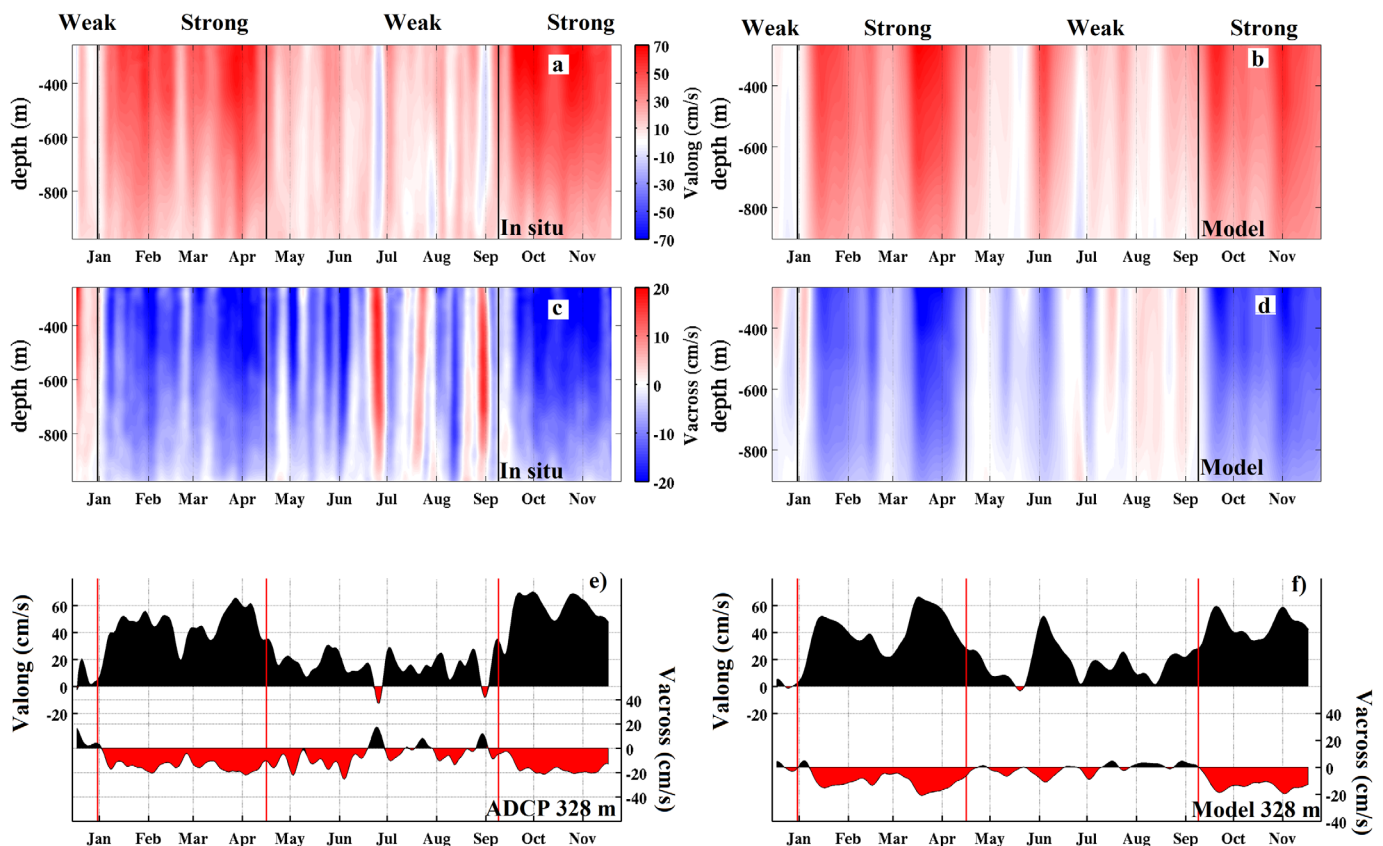
Figure 6. (a, b) Along-slope and (c, d) across-slope velocity time series recorded (left) by the ADCP and (right) from model outputs interpolated at the ADCP position during the mooring period (December 2014 to November 2015). Along-slope and across-slope velocity time series at 328 m (e) from the ADCP and (f) from model outputs interpolated at the instrument position for the mooring period (December 2014 to November 2015).
