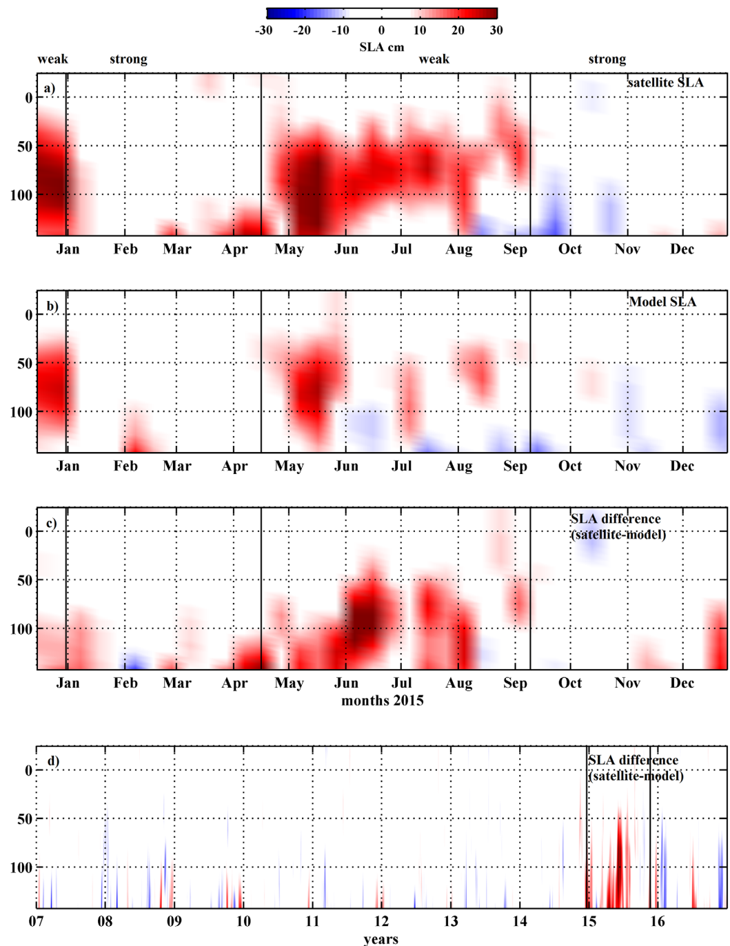
Figure 7. Hovmöller diagram of SLA (cm) along a 160 km-long section marked in red in Figure 1c (Jason track #26) based on (a) the along-track altimetric product from December 2014 to December 2015 and on (b) model outputs along the same track. (c) Difference between along-track SLA and model SLA. (d) Hovmöller diagram of the satellite minus model SLA over the same track #26 extended over the 10 year period of model availability (2007–2016).
