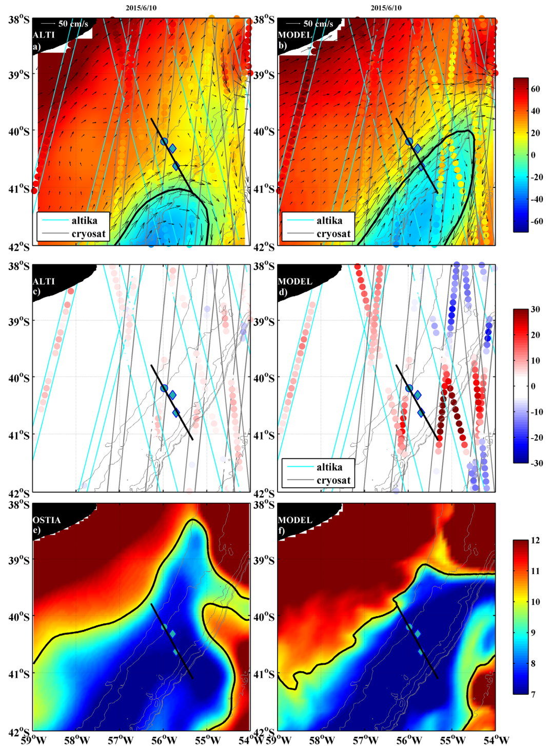
Figure 8. ADT distributions (in cm) from (a) gridded altimetric products and (b) model outputs for 10 June 2015. The along-track altimetric product (from Altika and Cryosat satellites) for the week centered on this date is superimposed. The differences between the gridded maps and the along-track altimetric product are shown in (c) and (d). SST distributions ( ^{\circ}\text{C} ) (e) from OSTIA and (f) from model outputs for 10 June 2015. The black contour is the 10^{\circ}\text{C} isotherm which corresponds to the location of the maximum SST gradient for that day. The black line indicates the position of Jason track #26. The position of the 2014–2015 moorings is indicated with green markers. Isobaths as in Figure 1.
