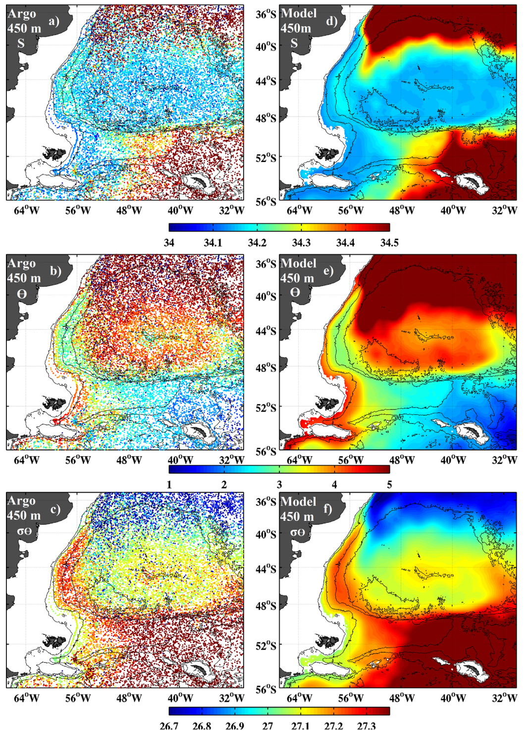
Figure 2. (a) Salinity (psu), (b) potential temperature ( ^{\circ}\text{C} ), and (c) potential density ( \text{kg}/\text{m}^3 ) at 450 m depth from Argo float profiles over the 2007–2016 period. (d) Mean salinity (psu), (e) potential temperature ( ^{\circ}\text{C} ), and (f) potential density ( \text{kg}/\text{m}^3 ) at 450 m depth over 2007–2016 from model outputs. Isobaths as in Figure 1.
