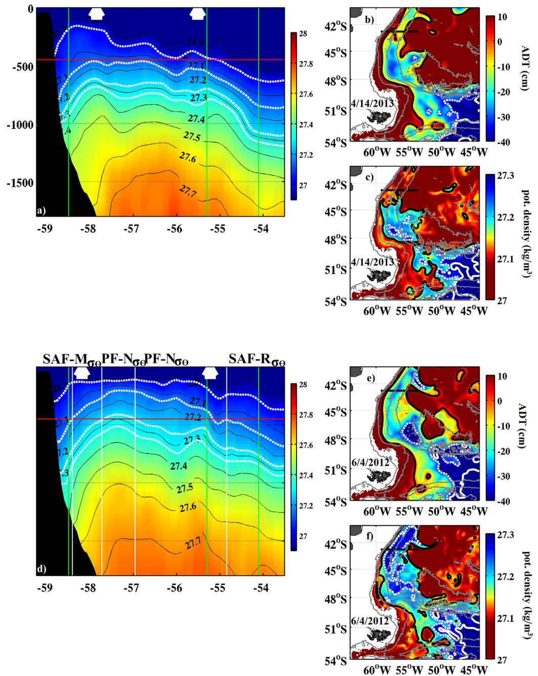
Figure 15. (a) Model potential density section at 43°S on 14 April 2013. The green vertical lines indicate the mean location of the SAF-M, SAF-R, and BCF according to the potential density (from Figure 13a). The thick white arrows near the surface indicate the location of the SAF-M and SAF-R according to ADT. 450 m depth is marked with a red line and dashed white lines are the selected isopycnals indicated in Table 3. (b, c) Model ADT and density maps for the 14 April 2013. (d) Same as Figure 15a for the 4 June 2012. The white vertical lines indicate the location of the SAF-M, PF-N, and SAF-R inferred from potential density at 450 m as labeled. (e, f) Model ADT and density maps for the 4 June 2012.
