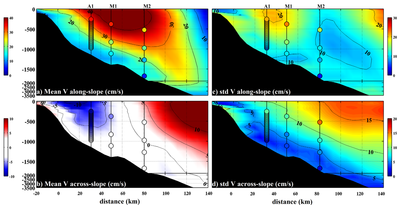
Figure 5. (a, b) Mean and (c, d) standard deviation of the (top) along-slope and (bottom) across-slope velocity components from model outputs (December 2014 to November 2015) along the 160 km-long section (from west to east) marked in red in Figure 1. Corresponding values from observations at each instrument are indicated by colored dots. The depth scale of the y axis is stretched in the upper 2,000 m.
