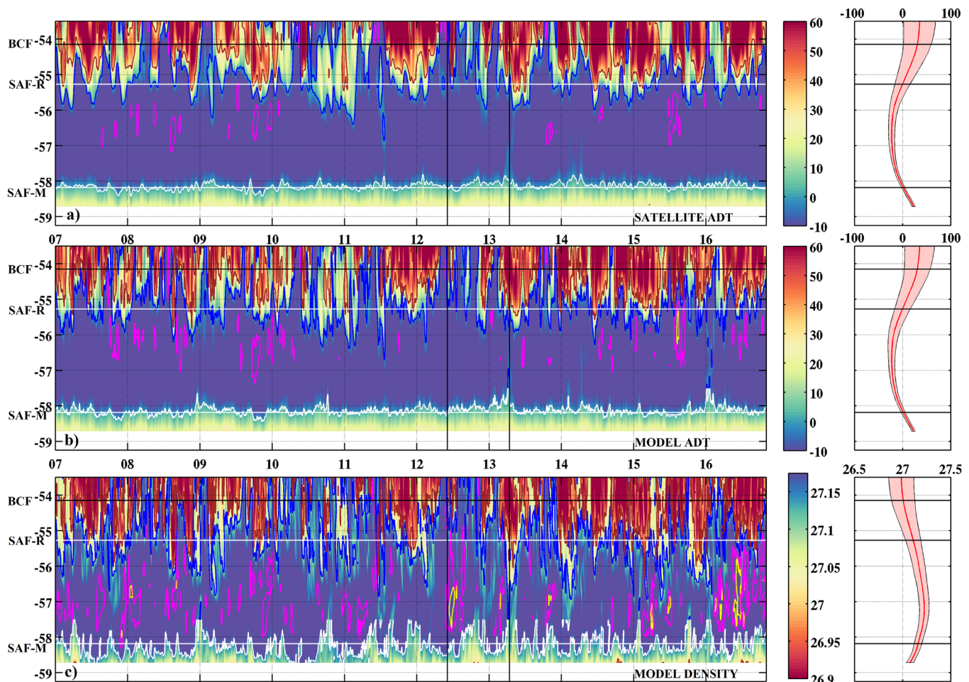
Figure 14. (left) Hovmöller diagrams of (a) satellite gridded ADT (in cm), (b) model ADT (in cm) and (c) model potential density (in \text{kg/m}^3 ) at 450 m along a zonal section (red line in Figure 10a) at \sim 43^\circ\text{S} . The mean locations of the SAF-M ( 58.3^\circ\text{W} ), the SAF-R ( 55.3^\circ\text{W} ), and the BCF ( 54.1^\circ\text{W} ) are indicated in each plot with horizontal lines. The isolines corresponding to the SAF-M are in white, to SAF-R in blue and to BCF in brown. In each plot, the pink and yellow contours correspond to PF-N and PF-M. The two vertical black lines mark the dates that are shown in Figure 15. (right) Mean value of each variable plotted along the section. Shaded area represents the standard deviation.
