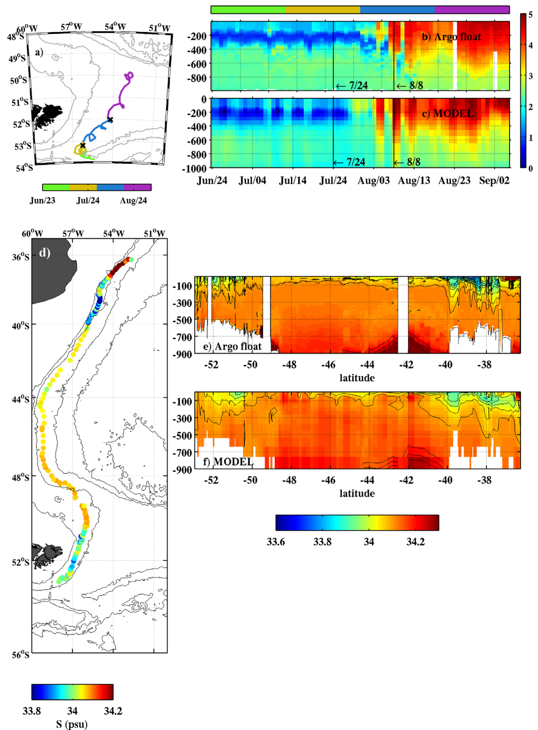
Figure 3. (a) Trajectory of Argo float 1 (platform number 6901650) colored as a function of time. Daily potential temperature profiles (b) from the Argo float and (c) collocated model outputs as a function of time. Black crosses in Figure 3a indicate the float position at the dates indicated with vertical lines in Figures 3b and 3c. (d) Trajectory of Argo float 2 (platform number 6901654) colored as a function of the observed salinity at 30 m. Isobaths as in Figure 1. (e) Salinity profiles from the Argo float with a daily resolution. (f) Salinity profiles from the model outputs with a daily resolution. Shallow topography appears in white. The x axis is latitude. The y axis is the depth (in m).
