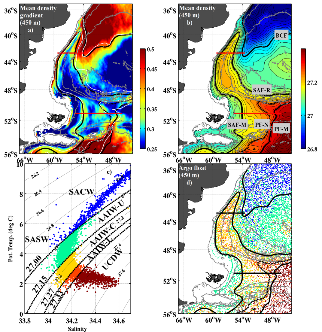
Figure 10. (a) Mean potential density gradient at 450 m in \text{kg/m}^3/100 \text{ km} from model outputs and (b) mean potential density ( \text{kg/m}^3 ) at 450 m. The heavy black contours correspond to specific fronts from Table 3. The thin white lines are the ADT contours of Figure 9a. (c) Potential temperature-salinity diagram from Argo float data at 450 m classified in terms of potential density criteria at 450 m (Table 3). Corresponding water masses are indicated. (d) Location of the Argo float profiles over 2007–2016. The color code corresponds to the potential density at 450 m as in Figure 10c. The heavy black contours are the potential densities isolines from Figure 10b. Isobaths as in Figure 1.
