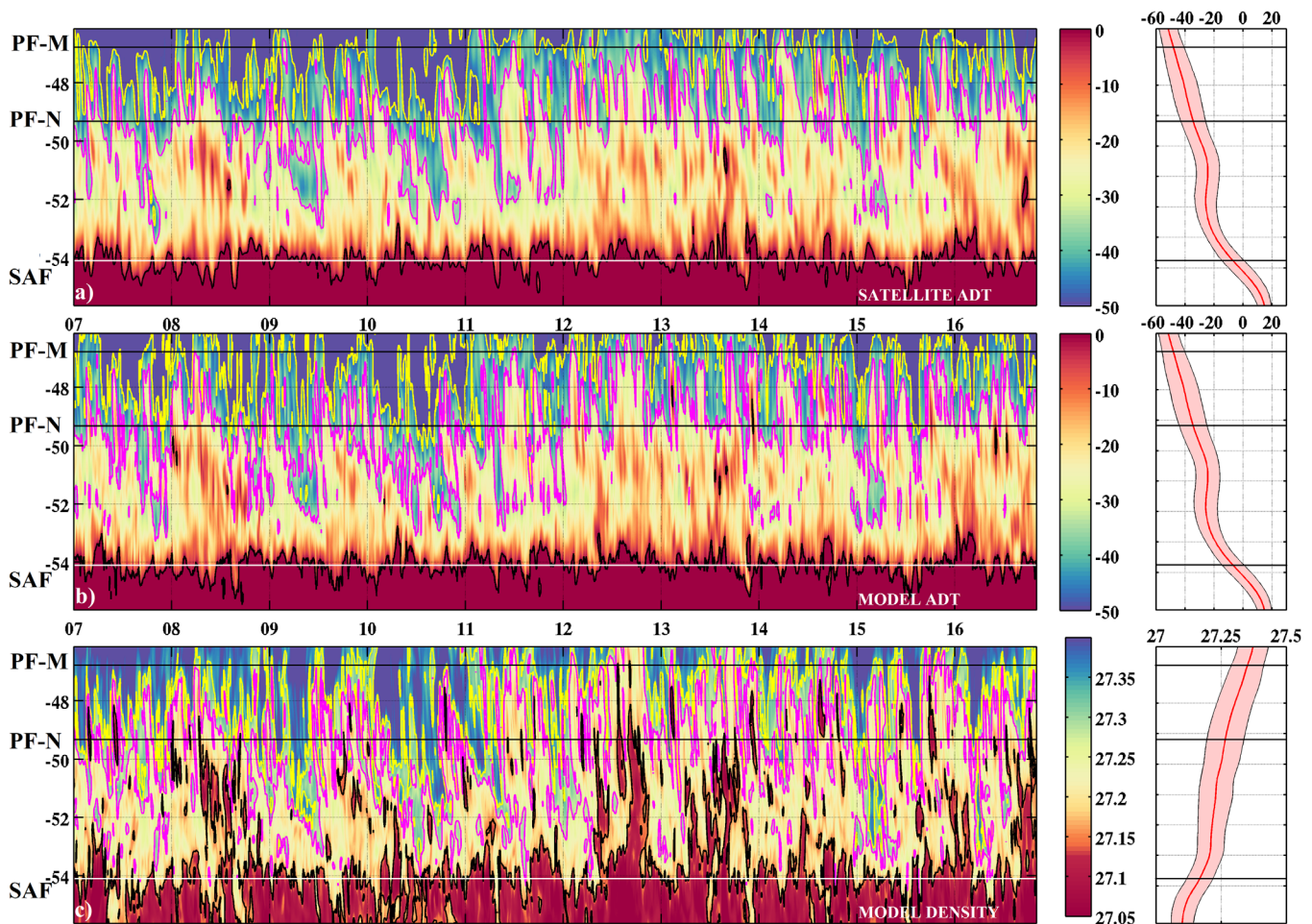
Figure 12. (left) Hovmöller diagrams of (a) satellite gridded ADT (in cm), (b) model ADT (in cm), and (c) model potential density (in \text{kg/m}^3 ) at 450 m along a zonal section (red line in Figure 10a) at \sim 51^\circ\text{S} over the Malvinas Plateau. The mean locations of the SAF-M ( 54.1^\circ\text{W} ), the PF-N ( 49.3^\circ\text{W} ), and the PF-M ( 46.8^\circ\text{W} ) are indicated in each plot with horizontal lines. The isolines corresponding to the SAF-M are in black, to PF-N in pink, and to PF-M in yellow. (right) Mean value of each variable plotted along the section. Shaded area represents the standard deviation.
