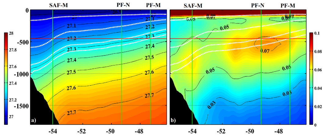
Figure 11. (a) Mean density and (b) standard deviation of potential density along the zonal section at 51°S (red line in Figure 10a). The mean position of SAF-M, PF-N and PF-M and the 450 m depth are indicated with green and red lines, respectively.
