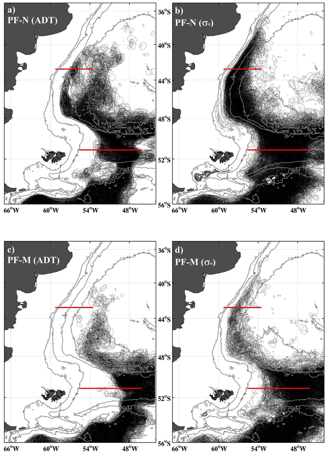
Figure 16. Loci of PF-N and PF-M from 10 years of model snapshots (sampled every 5 days). (a) Positions of PF-N from ADT. (b) Positions of PF-N from potential density at 450 m. (c) Positions of PF-M from ADT. (d) Positions of PF-M from potential density at 450 m.
