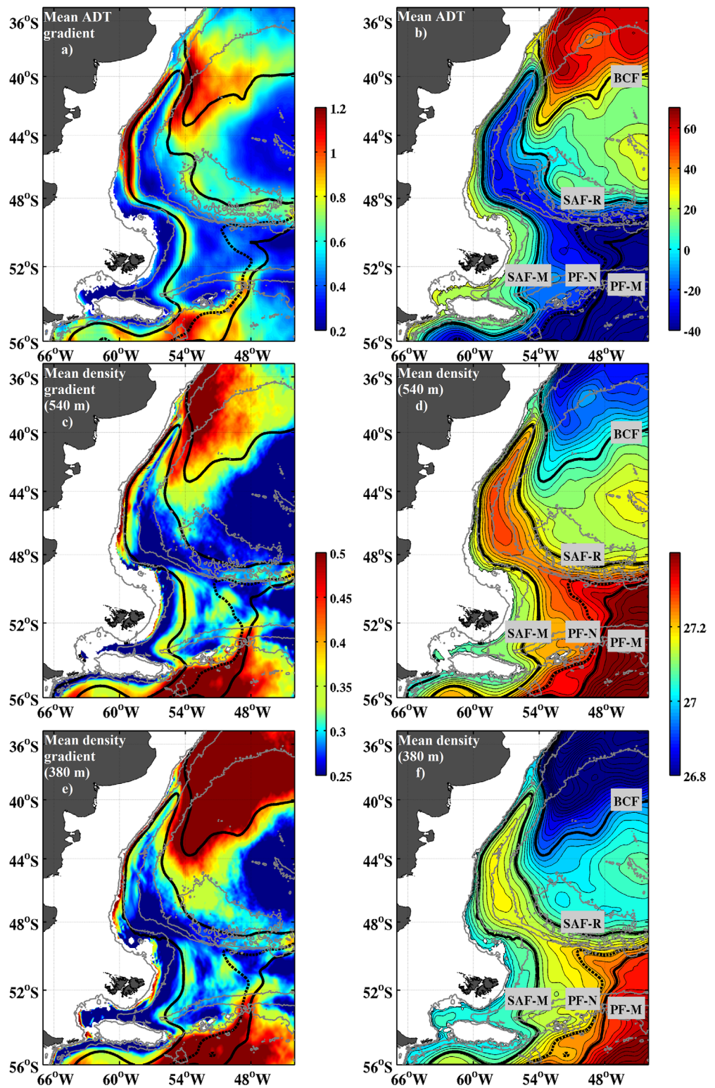
Figure 9. (a) Mean ADT gradient in cm/100 km from gridded altimetry and (b) mean ADT (in cm). (c) Mean potential density gradient at 540 m in kg/m 3 /100 km from model outputs and (d) mean potential density (kg/m 3 ) at 540 m. (e) Mean potential density gradient at 380 m in kg/m 3 /100 km from model outputs and (f) mean potential density (kg/m 3 ) at 380 m. The heavy black contours corresponds to specific fronts from Table 3. Isobaths as in Figure 1.
