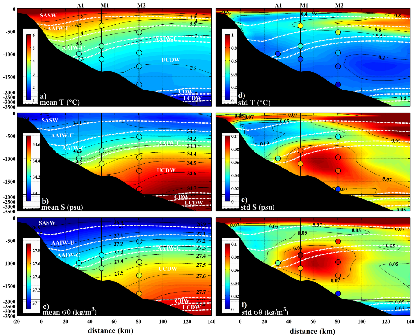
Figure 4. (a–c) Mean and (d–f) standard deviation of temperature (°C), salinity (psu), and density (kg/m 3 ) from model outputs (December 2014 to November 2015) along the 160 km-long section marked in red in Figure 1. Corresponding values from observations at each instrument are indicated by colored dots. The depth scale of the y axis is stretched in the upper 2,000 m.
