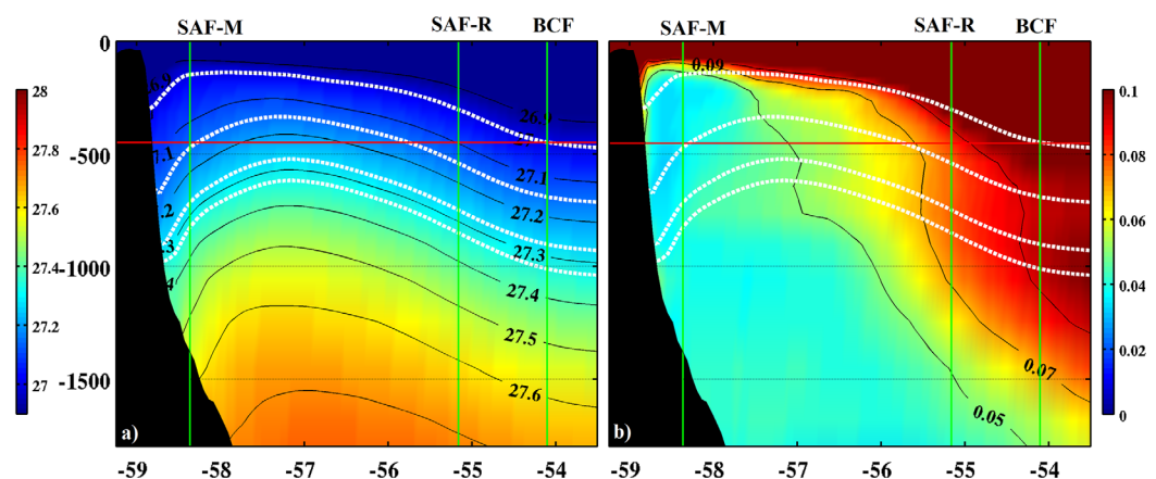
Figure 13. (a) Mean density and (b) standard deviation of density along the zonal section at 43^\circ\text{S} (red line in Figure 10a). The mean position of SAF-M, SAF-R, and BCF and the 450 m depth are indicated with green and red lines, respectively.
