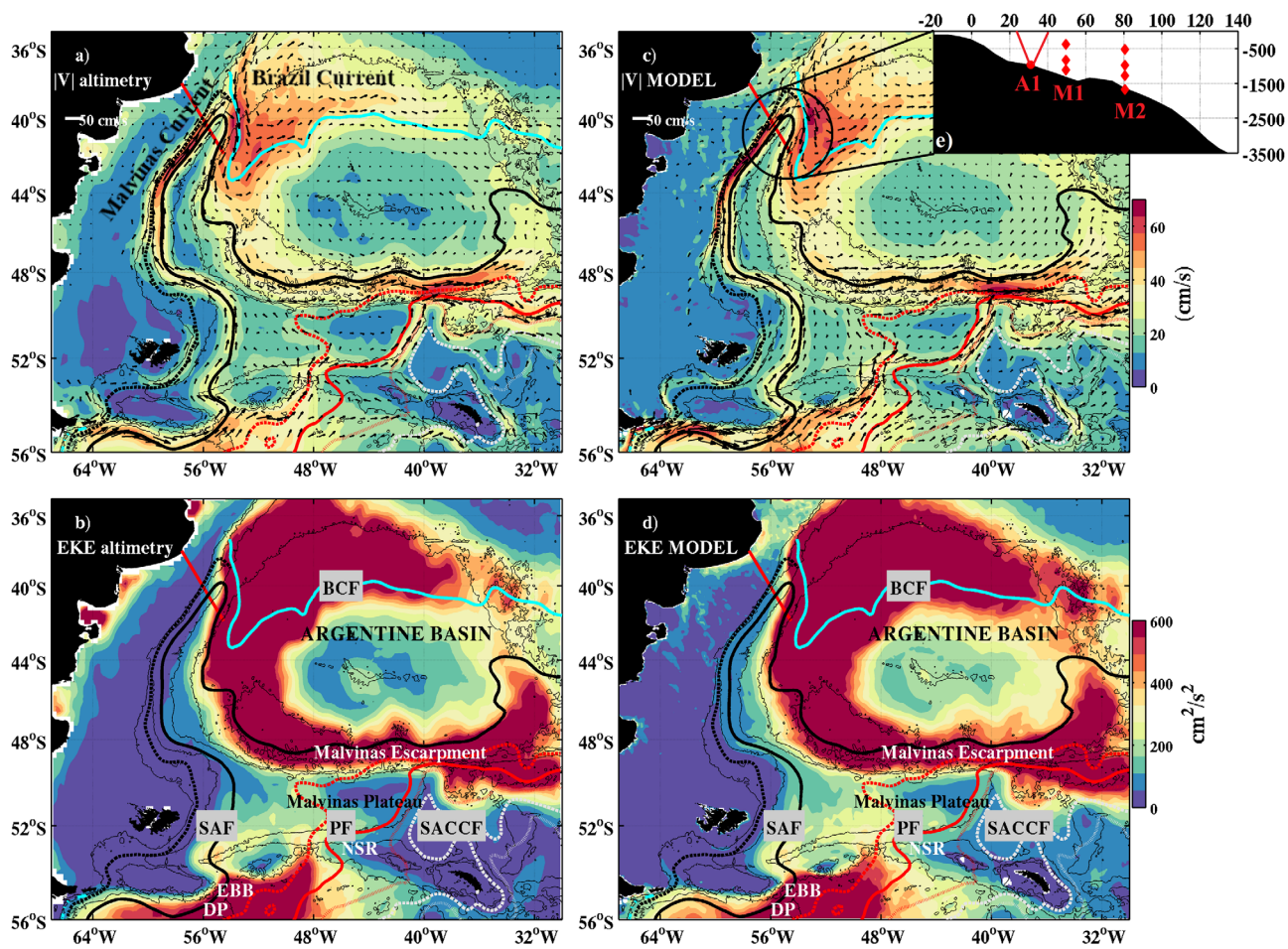
Figure 1. Mean surface velocity magnitude (in cm/s) and mean surface velocities (larger than 10 cm/s) (a) from gridded altimetry and (c) from model outputs. Mean eddy kinetic energy per unit mass (in \text{cm}^2/\text{s}^2 ) (b) from gridded altimetry and (d) from model outputs for the 2007–2016 period. Bottom topography isobaths correspond to 6,000, 5,000, 3,000, 1,000, and 300 m (from Smith & Sandwell, 1994). The mean locations of the main Antarctic Circumpolar Current (ACC) fronts as defined by Barré et al. (2011) are plotted: Subantarctic Front (SAF), in black (SAF-M solid line and SAF-N dashed line); Polar Front (PF), in red (PF-M solid line and PF-N and PF-S dashed line); and Southern ACC (SACCf) in grey (SACCf-N and SACCf-S in dashed lines). The mean position of the Brazil Current Front (BCF, solid light blue) is from Ferrari et al. (2017). The red line indicates a segment of the Jason satellite track #26. The instruments on the 2014–2015 moorings are represented with red diamonds in Figure 1e. The 0 km is referred to the 300 m isobath EBB, East of Burdwood Bank; DP, Drake Passage; NSR, North Scotia Ridge.
