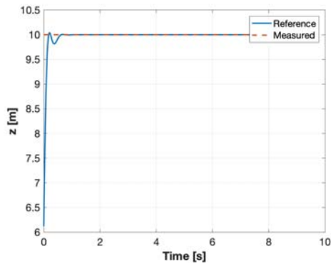
Fig. 7. Measured and reference value for the altitude for added mass
