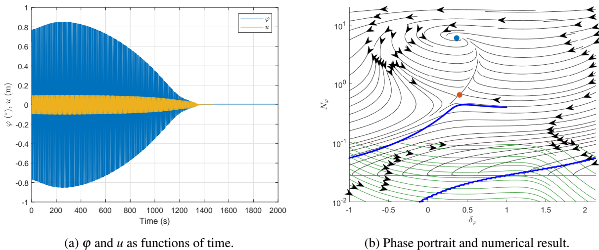
Figure 6 – Case 2: numerical result with NES, N_\varphi(0) = 0.4 \text{ s}^{-1} , \delta_\varphi(0) = 1 \text{ rad}
