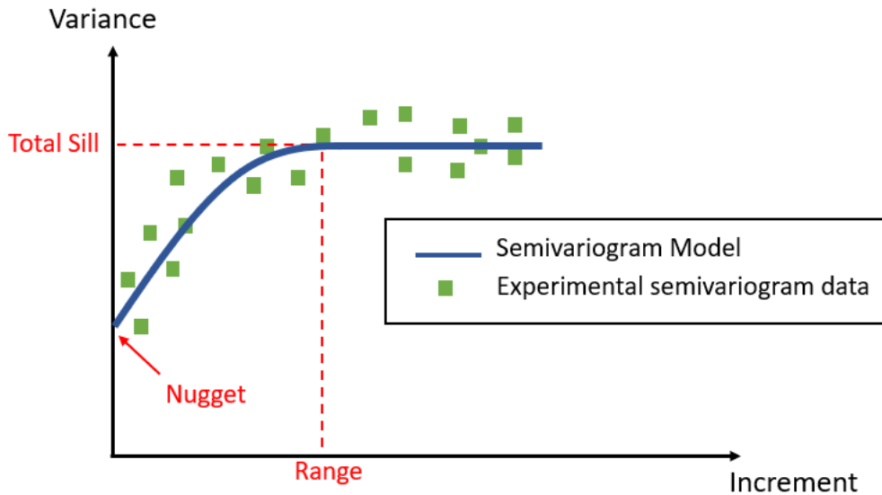
Figure 6 – Semivariogram model
