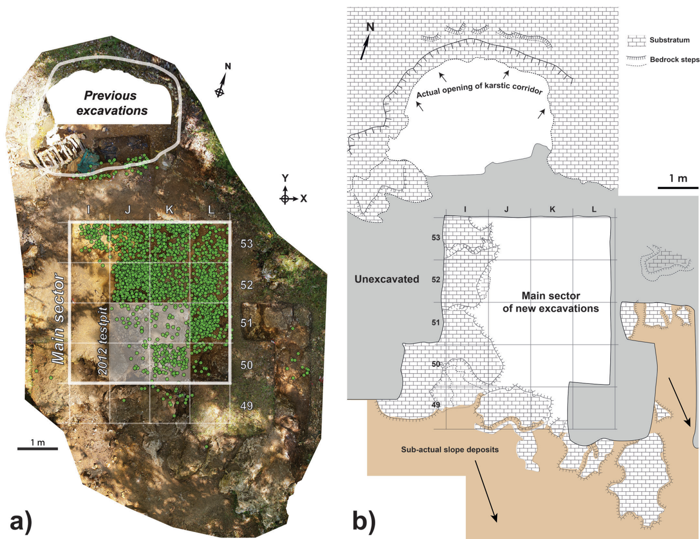
Figure 2. Top views of Cassenade with a) the extension of previous and new excavations (green circles: artifacts plotted in 2012 and 2013, background: orthophotography produced by photogrammetry, white rectangle: main sector, shaded grey: 2012 testpit); and, b) synthetic geomorphological map (opening of the karstic corridor, exposed bedrock, and slope deposits).
