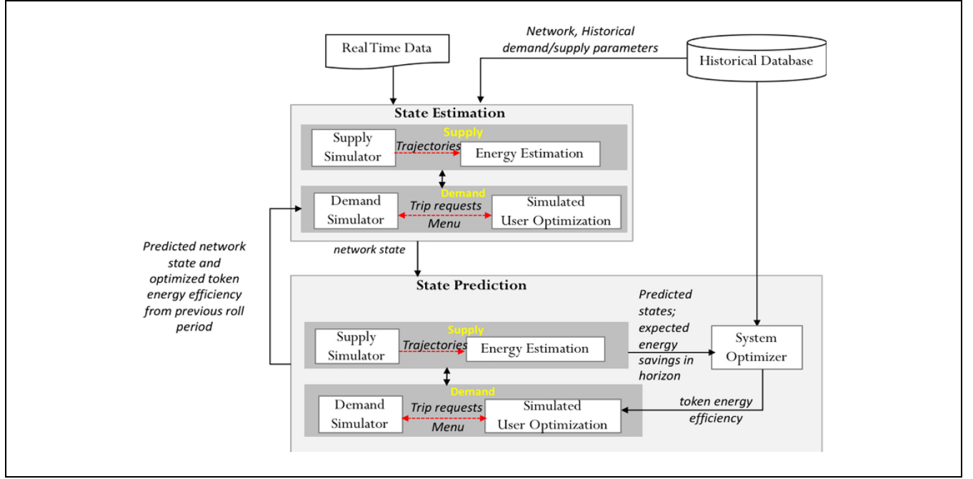
Figure 3. The System Optimization architecture.
