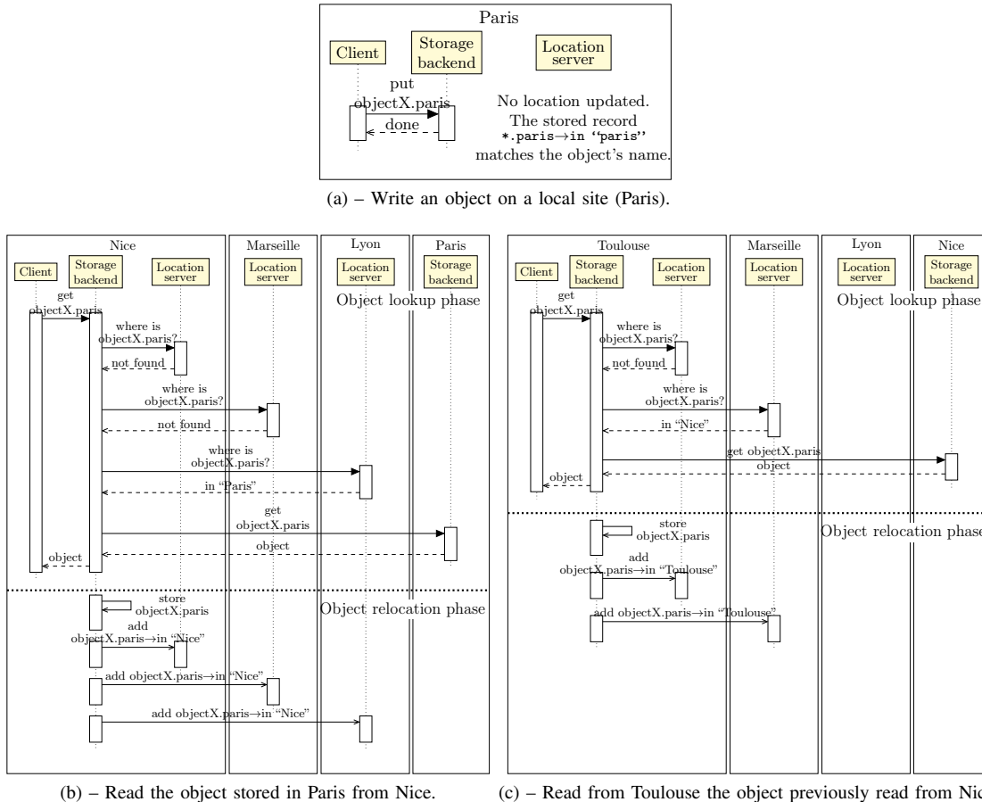
Fig. 9: Sequence diagrams of network traffic when a client writes an object in Paris and reads it first from Nice and secondly from Toulouse.
