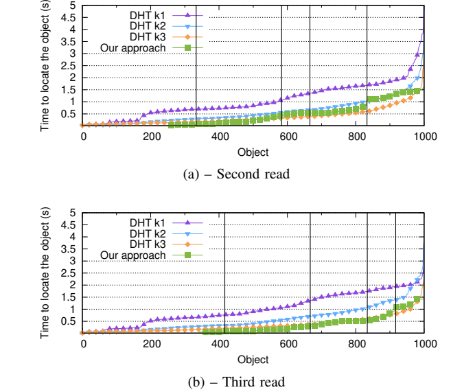
Fig. 14: Times to find the location of objects in the second read for all sites (a) and for the third read (b).
