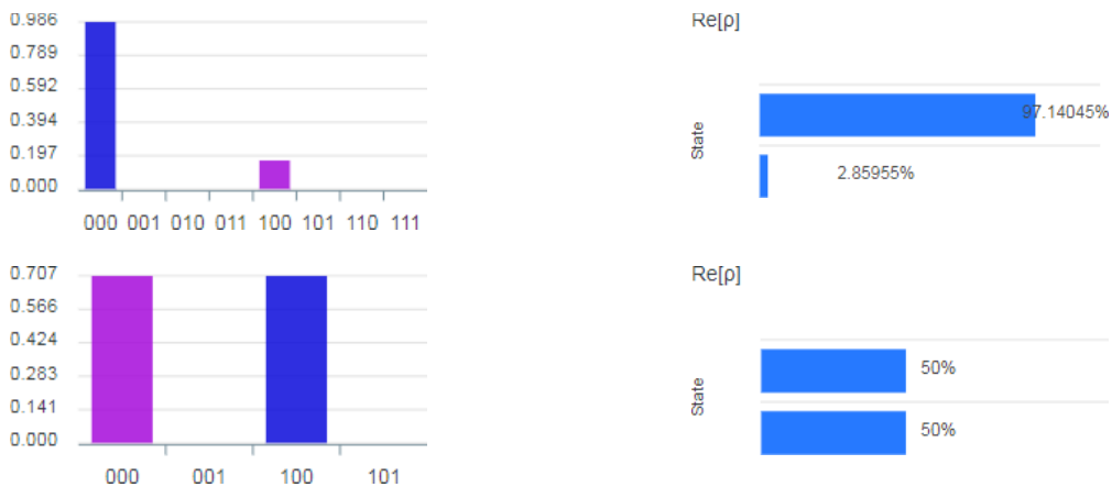
Figure 56 IBM Q delivers two types of outcomes in a randomly way, at the top: the wavefunction's complex modulus and the real part of the state with different values from those expected, and, at the bottom: wavefunction's complex modulus and the real part of the state, but with different values from those expected again.
