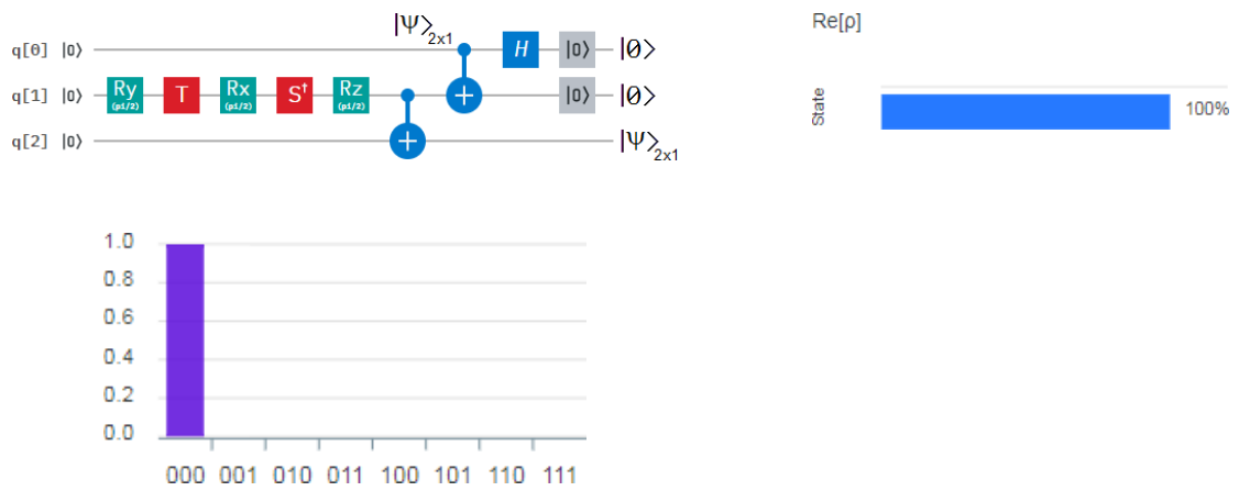
Figure 58 On the top-left is the quantum circuit for controlled quantum teleportation of |0\rangle via a not maximally entangled pair. On the bottom-left, the height of the bar is the complex modulus of the wavefunction. Finally, on the right is the real part of the state.
