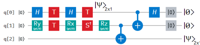
Figure 55 Controlled quantum teleportation protocol with a not maximally entangled pair.
