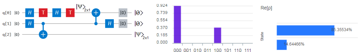
Figure 43 On the left is the quantum circuit for the qubit generation and the swapped BSC between q[0] and q[1]. In the middle, the height of the bar is the complex modulus of the wavefunction. On the right is the real part of the state (histogram o measurement probabilities).
