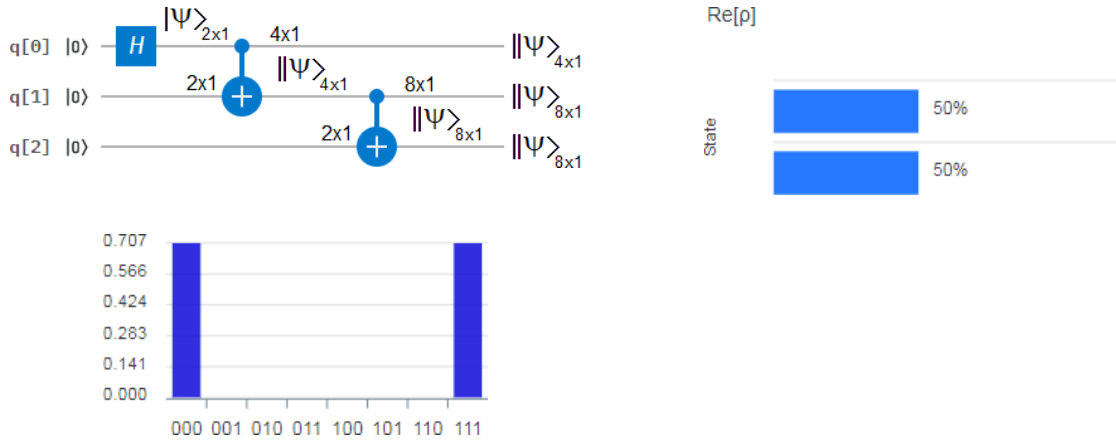
Figure 24 On the top-left is the quantum circuit for multiple entanglement generation thanks to two CNOT gates in cascade which produces three wavefunctions. Before and after each CNOT gate we can see the size of the statevector and the wavefunctions as vectors. On the bottom-left, the height of the bar is the complex modulus of the wavefunction. Finally, on the right is the real part of the state.
